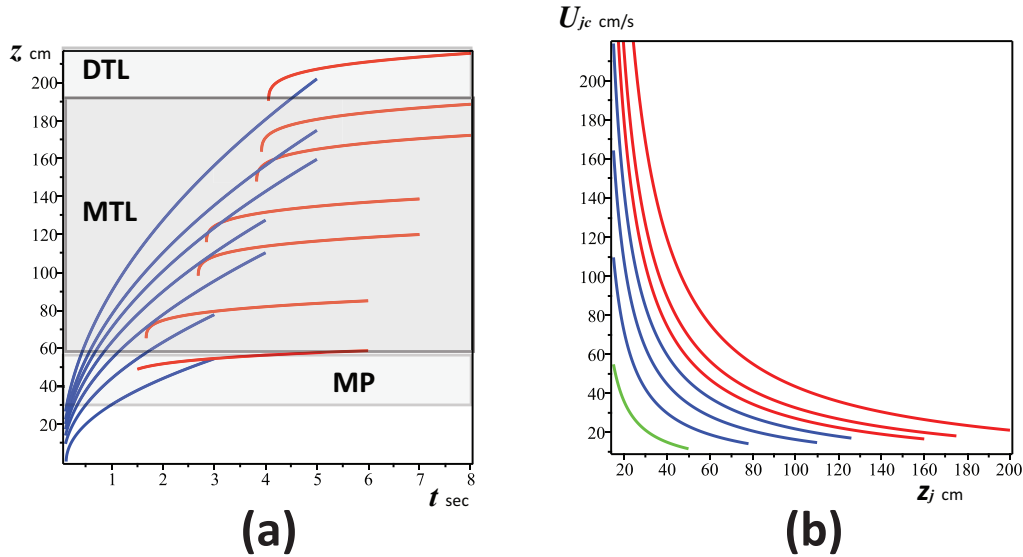
Figure 4: Jet/Puff horizontal displacement and centerline velocity. Panel (a) displays the displacement z_{jc} of the starting jet (blue) and z_{pc} of the puff (red) as functions of time from (equations (7)–(10)), for the three vaping topographies described in section 2.1: DTL (Direct to Lung), MTL (Mouth to Lung) and MP (Mouth Puffing). We assumed as injection (exhalation times) 3, 4 and 5 seconds. The initial velocities from top to bottom are U_0 = 50, 100, 150, 200, 250, 300, 400 cm/s. Panel (b) depicts centerline velocities U_c for the starting jet (equation (8)), as functions of the horizontal displacement z_{jc} during the injection times and initial velocities of panel (a) (green for MP, blue for MTL and red for DTL). Notice that once injection stops the jet has reached velocities comparable to those of indoor air currents.
