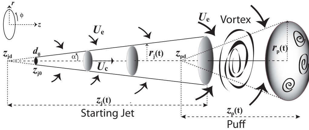
Figure 2: Puff and initial Jet with axial symmetry. The starting jet is propelled by linear momentum parallel to the centerline velocity U_c , the arrows above and below represent the entrainment velocity mixing surrounding air with the carrier fluid. As the fluid injection terminates (end of exhalation), the entrained air makes about 40 % of the fluid mass making the transition into a ellipsoidal puff through highly turbulent vortex structures. At this point the puff is likely to disperse rapidly as horizontal displacement velocities are comparable to velocity fluctuations characterizing high turbulence and thermal buoyancy.
