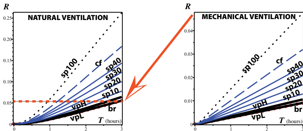
Figure 6: Infection risk in a restaurant. The same abbreviations as in figure 5 plus sp100 (speaking 100 % of the time, a possible outcome when spending 3 hours in a restaurant). As in figure 5, mechanical ventilation (air exchange rate 9.6/h) achieves a dramatic reduction of R and the curves for the risks from vaping are practically indistinguishable from the curve of the control case scenario of rest breathing (red circles).
