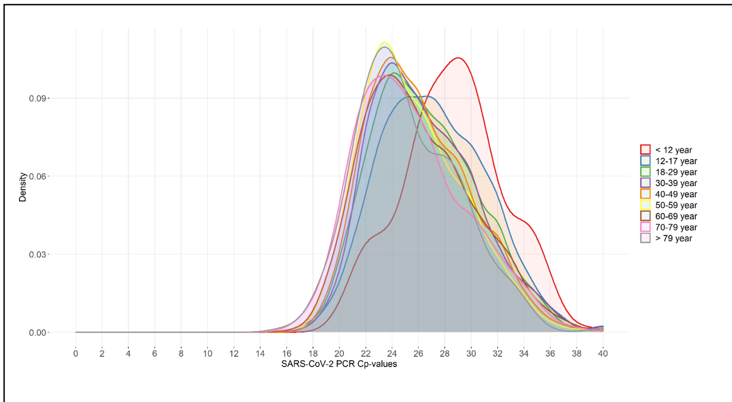
Figure 3. Distribution of SARS-CoV-2 PCR Cp-values within different age groups (n=18.290)
