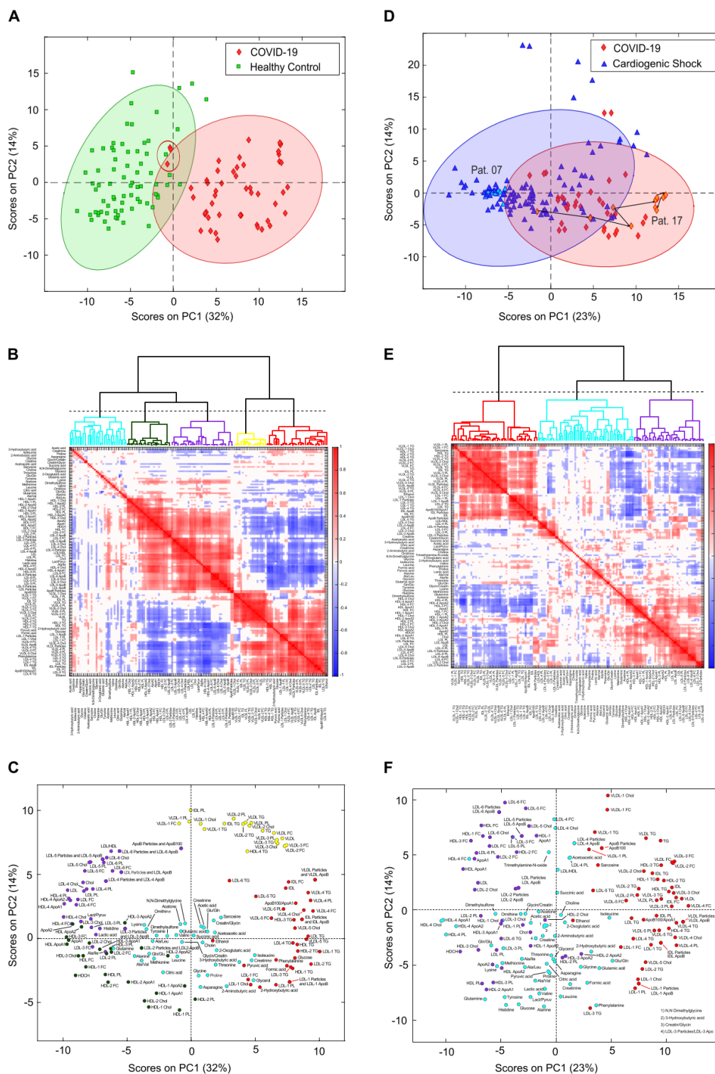
Figure 2. Targeted principal component and cluster analysis for IVDr NMR data. A. Scores plot of COVID-19 samples (red) vs Healthy Controls (green) showing almost perfect separation of the two groups. B. Corresponding hierarchical clustering of correlations for the loadings plot ( C ) of the same PCA showing groups of correlated metabolites and lipoproteins. D. PCA scores plot of COVID-19 (red) vs Cardiogenic Shock samples (blue) showing partial separation of the two groups. E. Corresponding hierarchical clustering of correlations for the loadings plot ( D ) of the same PCA showing groups of correlated metabolites and lipoproteins.
