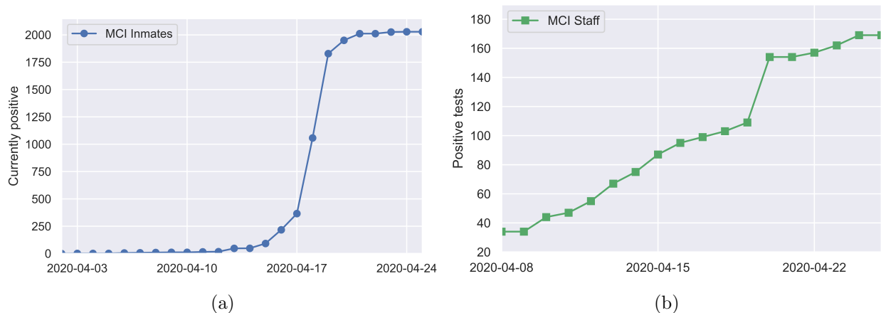
Figure 1: Positive tests over time among (a) inmates and (b) staff at MCI, as reported in [2].
