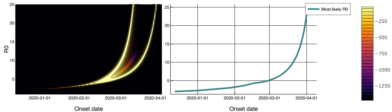
Figure 3: Left. Log-likelihood in the \mathcal{R}_0 -outbreak onset date plane, for mass testing data under a SEIR model with three week test-positive window following infectious onset. Right. \mathcal{R}_0 values that maximize the likelihood as a function of outbreak onset date. This curve corresponds to following the right-most branch of the ‘wishbone’ in the likelihood plot.
