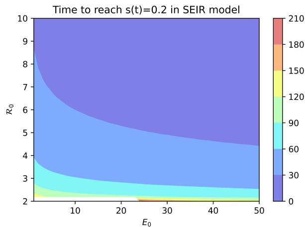
Figure 2: Time to infect 80% of population in SEIR model with median incubation period of 5.1 days [12] and mean infectious period of 5.6 days.
