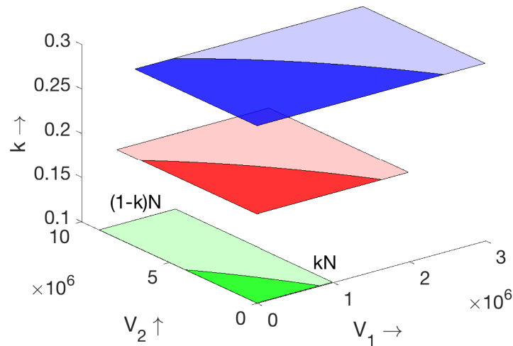
Figure 1: Regions of epidemic growth and extinction are marked with deep and light colours, respectively. Parameter values are \beta_{11} = 4 , \beta_{22} = 1 , \beta_{12} = \beta_{21} = 2.5 , \sigma_1 = \sigma_2 = 1 and k = 0.1 (green), k = 0.2 (red) and k = 0.3 (blue).
