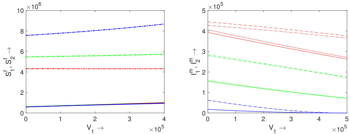
Figure 2: Left panel: analytical and numerical values of the final sizes of epidemic for two groups for k = 0.1 (blue), k = 0.2 (green), k = 0.3 (red). Right panel: analytical and numerical values of maximum number of infected individuals for two groups for k = 0.1 (blue), k = 0.2 (green), k = 0.3 (red). Other parameter values are as follows: \beta_{11} = 4 , \beta_{22} = 1 , \beta_{12} = \beta_{21} = 2.5 , \sigma = 1 , V_2 = 2.4 \cdot 10^6 - V_1 .
