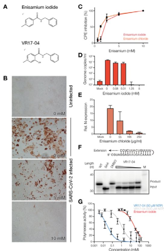
659 660 Figure 1. Enisamium inhibits SARS-CoV-2 infection and replication in vitro . (A) 661 Chemical structures of FAV00A and VR17-04. The chemical structure of FAV00B is 662 identical to FAV00A except that chloride ions are present instead of iodide. (B) 663 Inhibition of SARS-CoV-2 N expression in Caco-2 cells by enisamium chloride. (C) 664 Inhibition of SARS-CoV-2 cytopathic effect in Caco-2 cells by enisamium iodide and 665 chloride. (D) Quantification of SARS-CoV-2 RNA genome levels in NHBE cells 666 infected with SARS-CoV-2 after treatment with enisamium iodide. (E) Quantification 667 of HCoV-NL63 N mRNA levels in NHBE cells infected with HCoV-NL63 after 668 treatment with enisamium chloride. (F) Inhibition of the SARS-CoV-2 nsp12/7/8 RNA 669 polymerase complex by VR17-04 on a hairpin template. A mutant containing a 670 double amino acid substitution in the nsp12 active site (SDD=>SAA) was used as 671 negative control. DMSO was used as solvent control. (G) Quantification of SARS- 672 CoV-2 nsp12/7/8 RNA polymerase complex inhibition by enisamium or VR17-04 on 673 a hairpin template. For VR17-04 two nucleotide triphosphate concentrations were 674 used. Polymerase activity was plotted against drug concentration and dose-response 675 curves were fit to the data. Quantification is from n=3 independently prepared 676 reactions using the same nsp12/7/8 protein preparation. Error bars represent 677 standard deviation.
