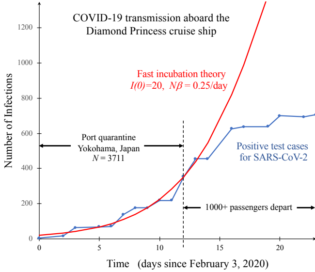
Fig. S1. Validation and calibration of the fast-incubation model for the super-spreading event on board the Diamond Princess cruise ship, during its twelve day quarantine at Yokohama, Japan in February 2020 (30). Fitting the number of SARS-CoV-2 positive cases versus time (blue data points) during the quarantine period, to the fast-incubation solution of the SEI model, Eq. [6], (red curve) yields estimates for the initial number infected ( I_0 = 20 ) and the transmission rate ( N\beta = 0.25/\text{day} ), from which we infer the concentration of infection quanta from breathing ( C_q = 30 quanta/ \text{m}^3 ). The relevant physical parameters are listed in Table S1.
