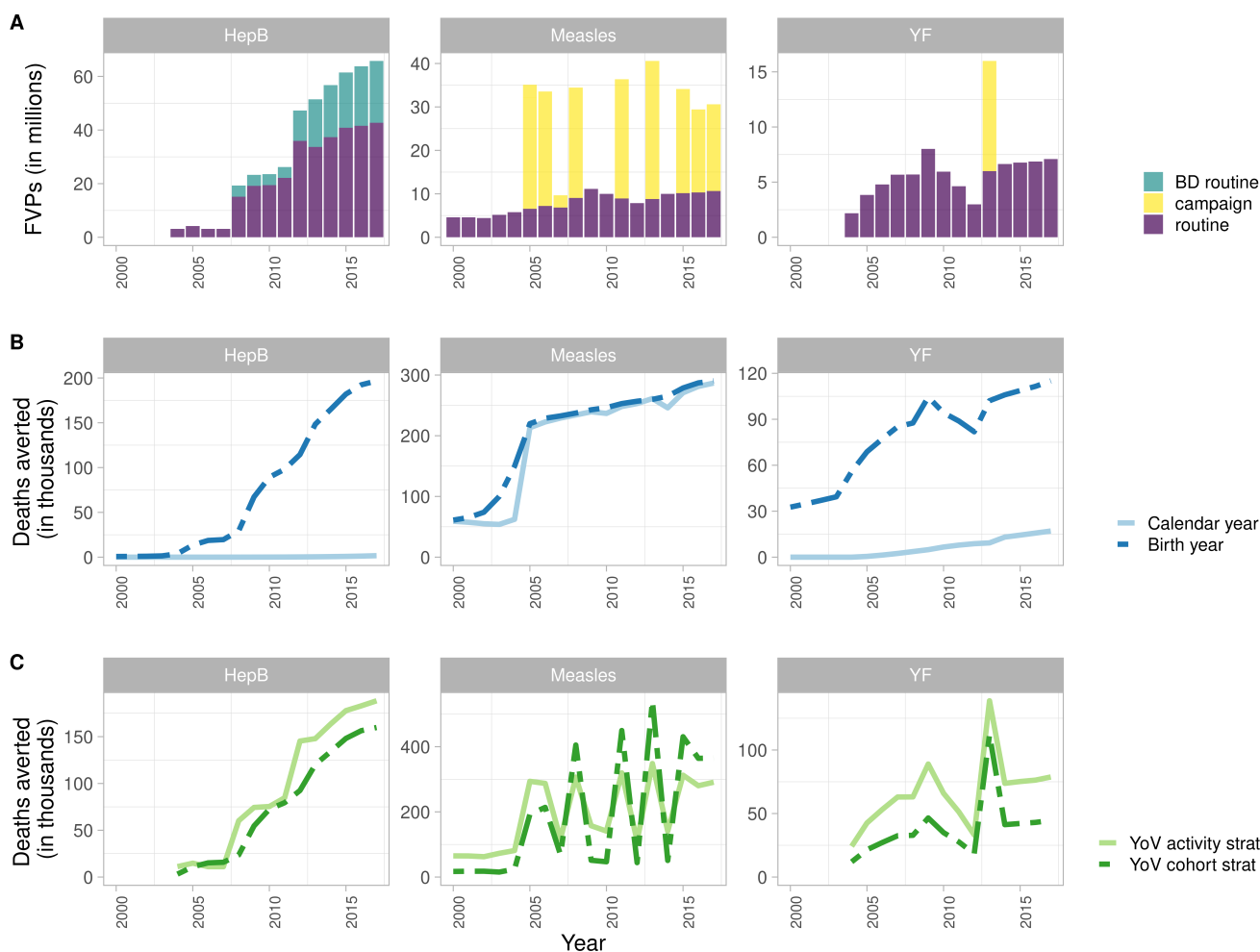
Figure 1. Fully vaccinated persons (FVPs) and mean estimates of deaths averted for Hepatitis B (HepB) in Country A, measles in Country B and yellow fever (YF) in Country C from 2000 to 2017. (A) FVPs for HepB birth dose (BD routine) and infant dose (routine) routine vaccination activities. FVPs for first routine dose of a measles containing vaccine and measles campaign activities. FVPs for YF routine and campaign activities. (B) Impact by calendar and birth year methods. (C) Impact by year of vaccination (YoV) with impact ratio stratified by activity type and birth cohort.
