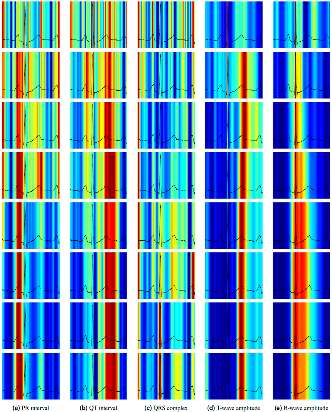
Figure S3. Attention maps from intermediate convolutions. First row is last convolution in the first residual block, second row is last convolution in second residual block etc.
