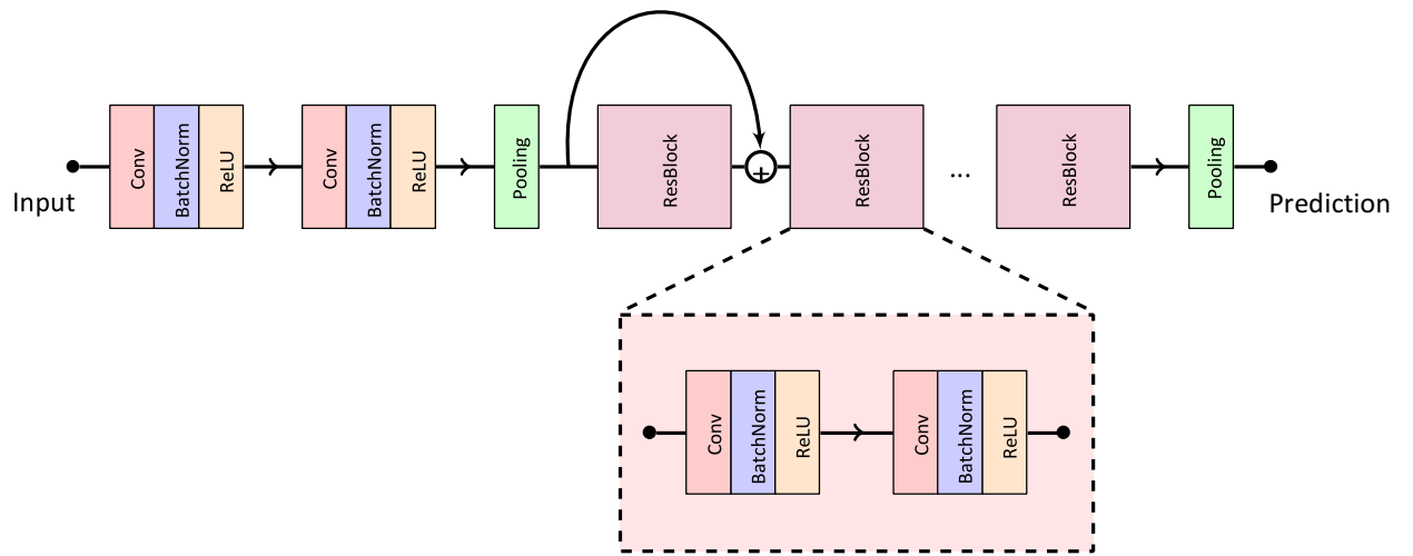
Figure S2. The convolutional neural network-based architecture used for all experiments.
