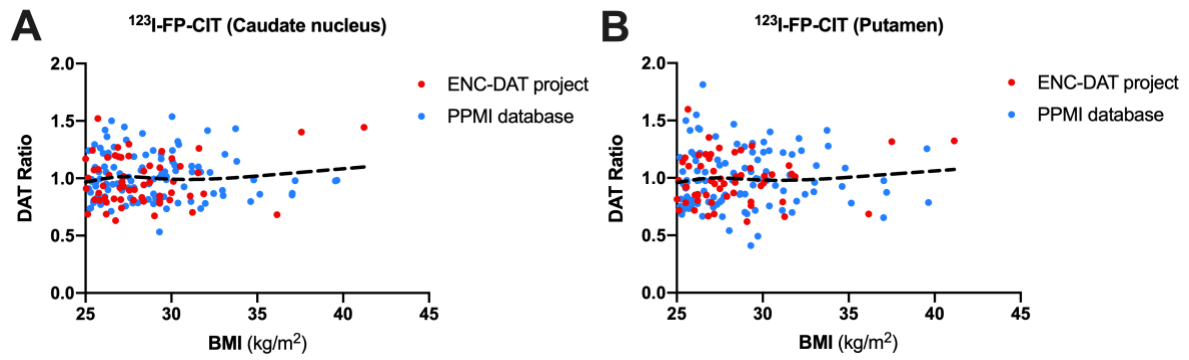
Figure 3. Scatter plots and spline curves of DAT ratio and BMI; A. Caudate nucleus; B. Putamen
