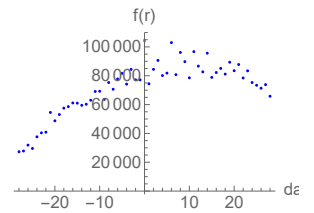
lag 8 in [7,11]
