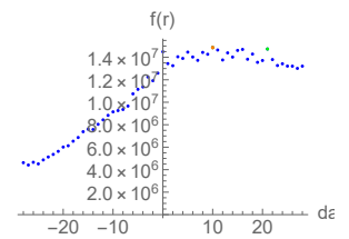
lag 11 in [9,16]
