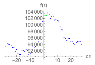
lag 5 in [3,8]
