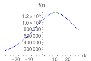
lag 10 in [9,12]
