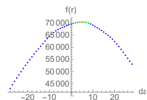
lag 4 in [1,8]
