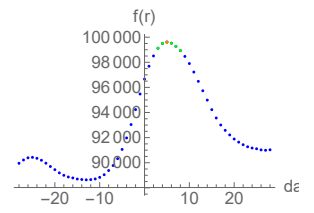
lag 5 in [3,8]
