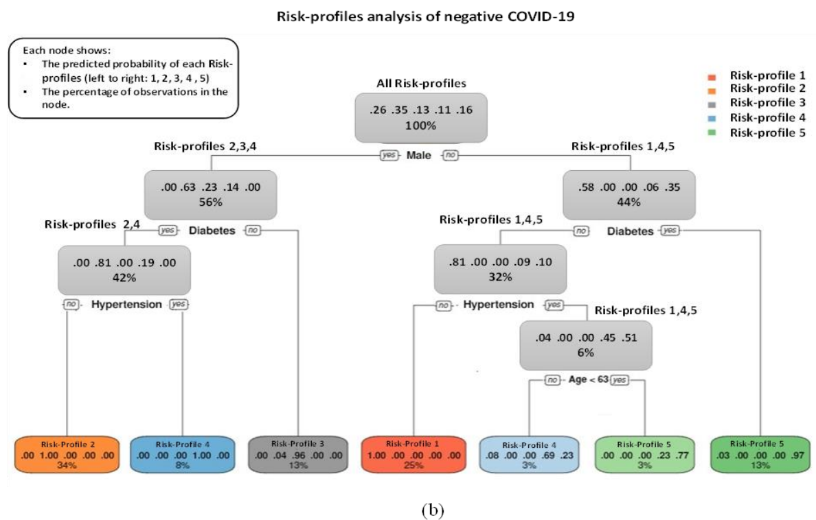
Fig. 5. Decision Trees of discovered risk-profiles for, (a) hospitalized infected patients, (b) hospitalized non-infected cases.
