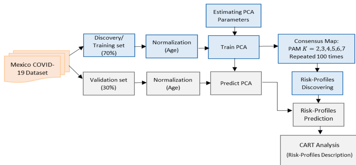
Fig. 2. The overall methodology of risk-profile's classification of Mexico COVID-19 data set. The multimodal data is split into training and testing sets and the results of the testing set are used to describe the association of disease risk-profiles to clinically relevant outcomes.
