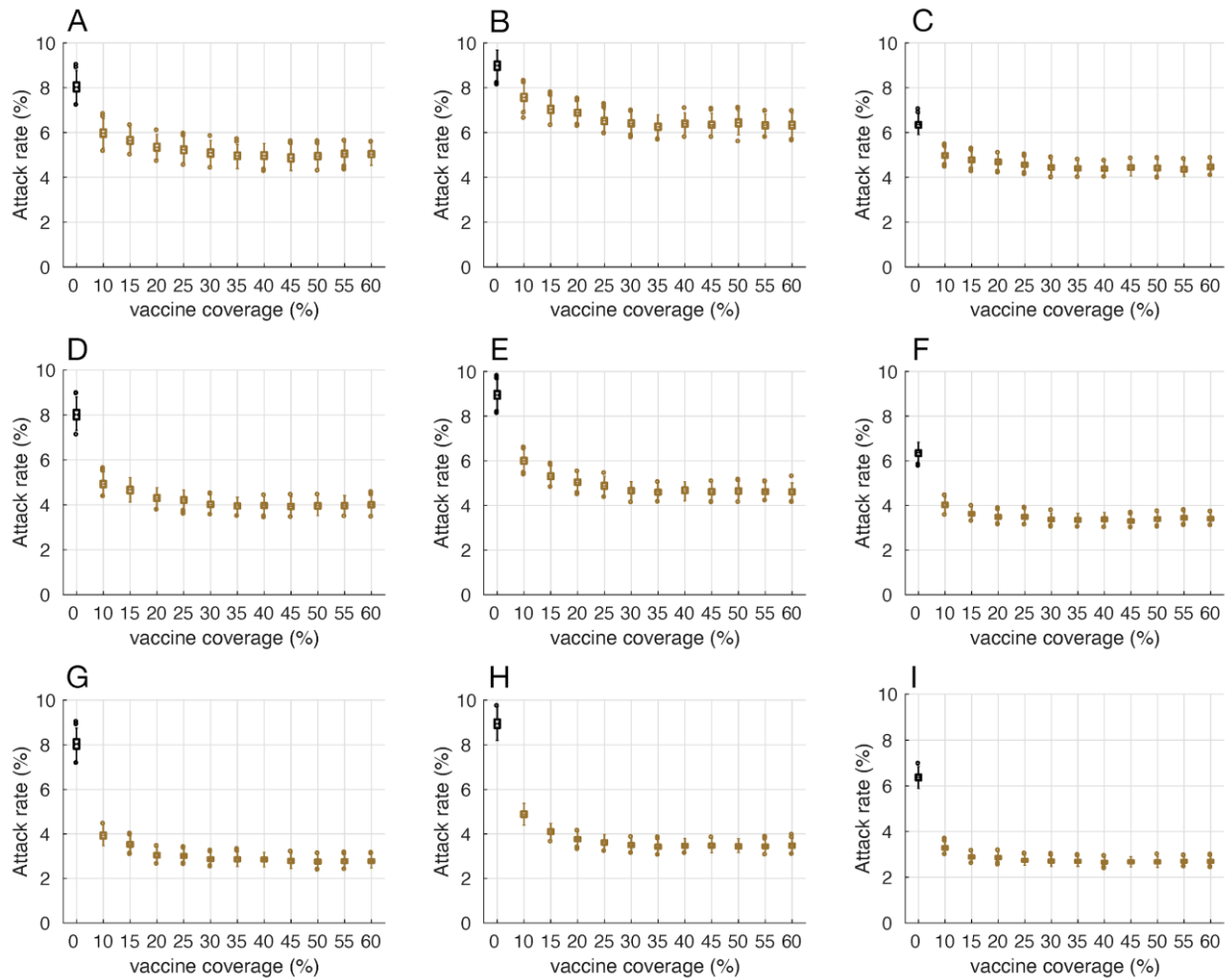
Figure A9. Projected attack rates with 5% (A,D,G), 10% (B,E,H), and 20% (C,F,I) pre-existing immunity and different vaccination coverage in the range 10-60%. The protection efficacy of vaccines against infection is 0% (A,B,C), 50% lower than the efficacy against disease (D,E,F), and the same as efficacy against disease (G,H,I). Vaccine efficacy was reduced by 10-50% among vaccinated elderly and comorbid individuals.
