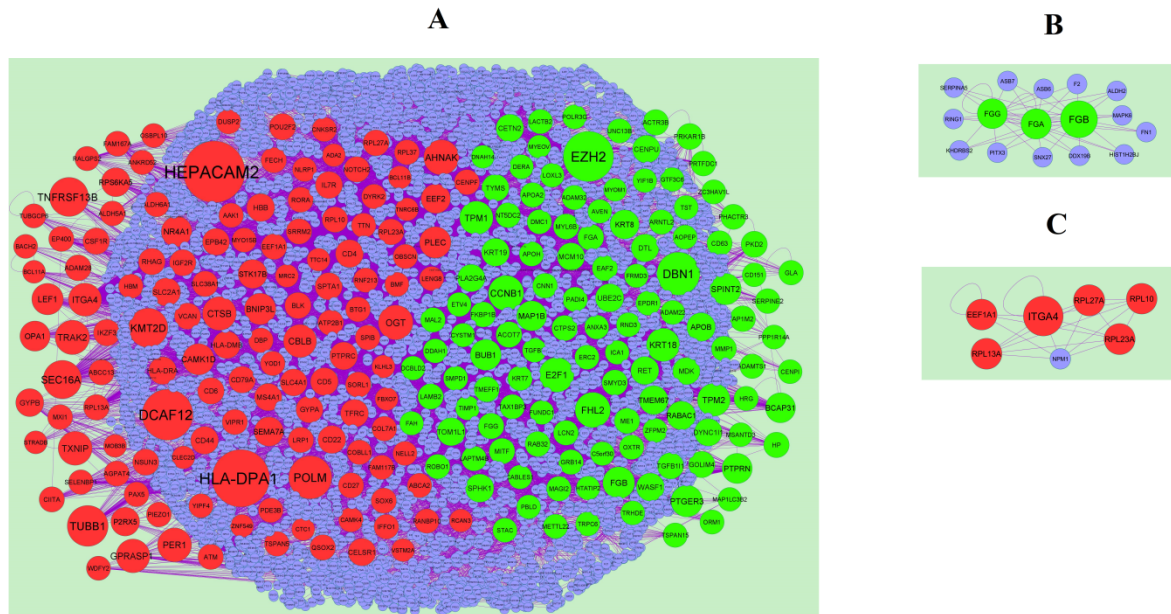
Fig. 3. PPI network and the most significant modules of DEGs. (A) The PPI network of DEGs was constructed using Cytoscape (B) The most significant module was obtained from PPI network with 16 nodes and 44 edges for
