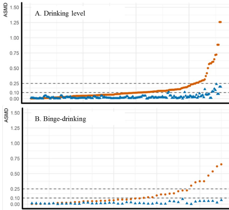
Supplemental Figure S3.4. Absolute standardised mean differences (ASMD) in pairwise between-group contrasts (e.g. ASMD_{AGE} abstinent vs. light drinkers, ASMD_{AGE} abstinent vs. moderate drinkers, etc.) before (red circle) and after (blue triangle) propensity score weighing. On the X-axis, contrasts are ordered by their pre-weighting ASMD. Dashed horizontal lines indicate acceptable ( ASMD < 0.1 ) and adjustable ( ASMD < 0.25 ) residual imbalance after weighing. No residual between-group difference exceeds ASMD = 0.25 .
