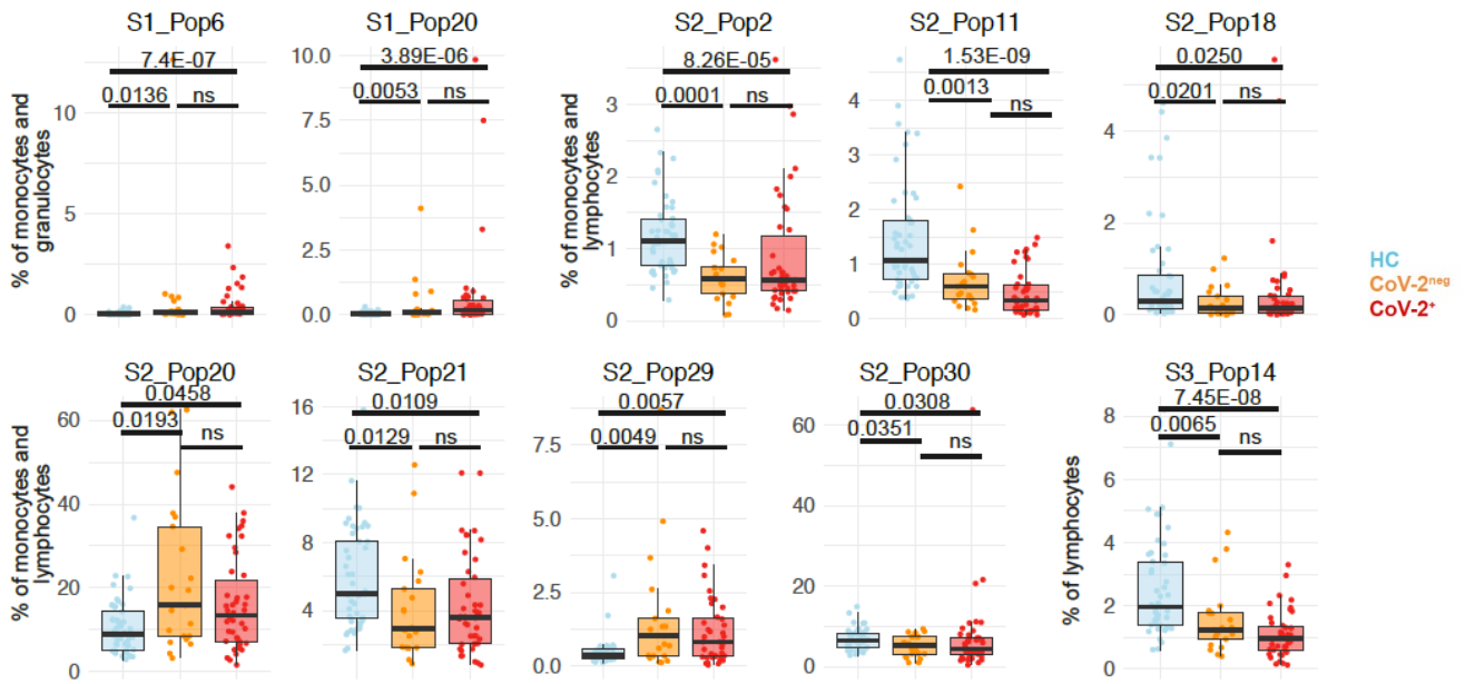
Supplemental Figure 2. Populations altered in hospitalized patients identified by data-driven (unbiased) analysis. Box and Whisker plots showing frequencies of selected immune cell populations dysregulated in hospitalized patients compared to healthy controls (HC); SARS-CoV-2 + (CoV-2 + , red) compared to SARS-CoV-2 neg (CoV-2 neg , yellow) and HC (blue) (HC n = 49 ; CoV-2 neg n = 21 ; CoV-2 + n = 42 ). Mann-Whitney U test (for n = 2 categories) and Kruskal-Wallis test (for n > 2 categories) followed by a Dunn's post hoc-test were used. ns: not significant.
