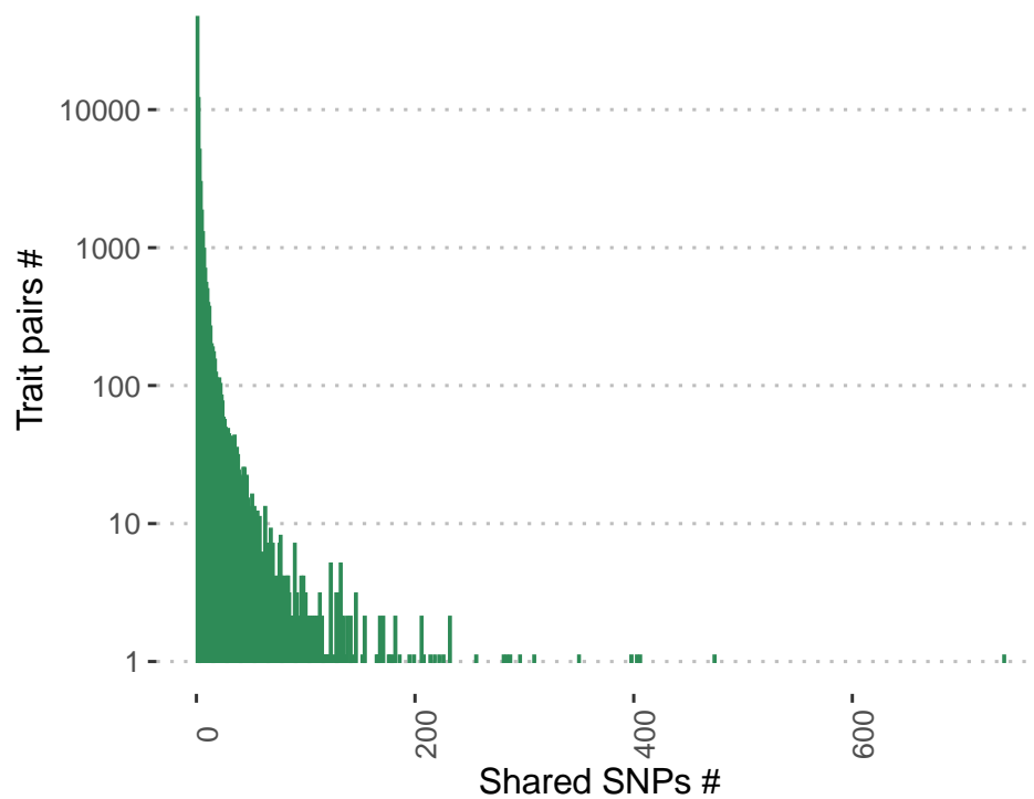
Figure S2. Histogram of shared SNPs for each trait pair in NHGRI-EBI GWAS catalog from iCPAGdb at false discovery rate of 0.1. Among 76127 trait pairs (including compound phenotypes), the mean number of shared independent SNPs was 3.10, and 38.8% of trait pairs shared more than 1 SNP. “Mathematical ability” and “self reported educational attainment” shared the most SNPs with 739.
