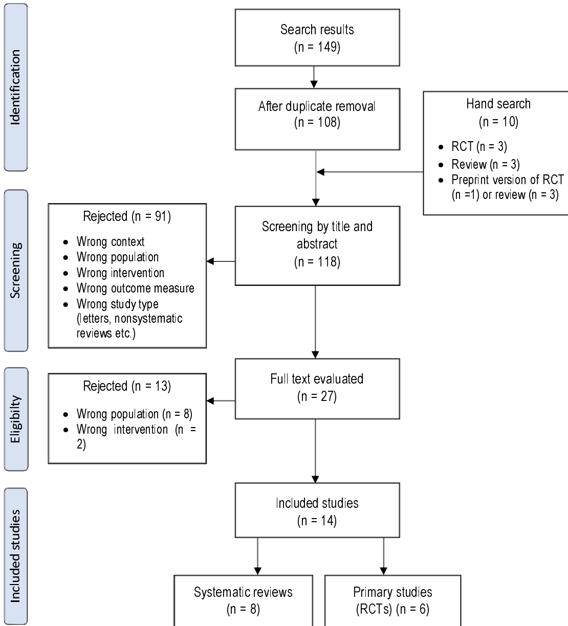
Figure 1: PRISMA flowchart.
