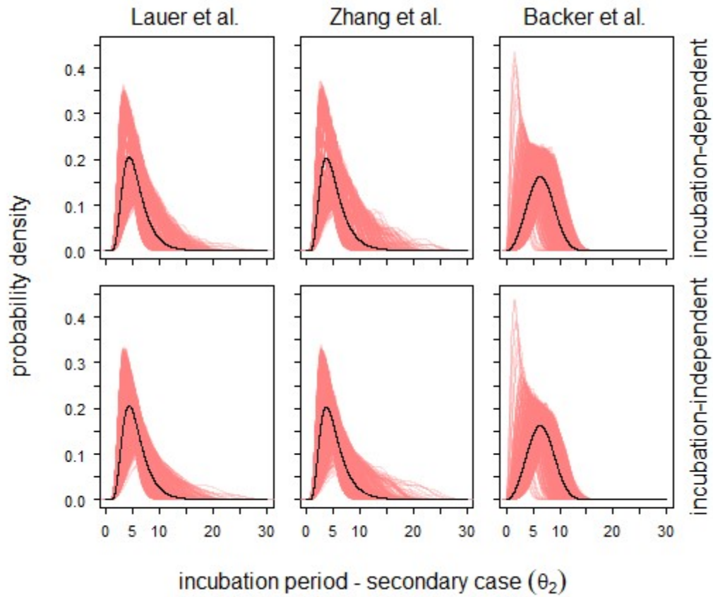
Fig. S4 Overlaid posterior distributions for the incubation period of the secondary case ( \theta_2 ) of each case pair in the post-lockdown period. Black lines show the incubation period prior for each analysis.
