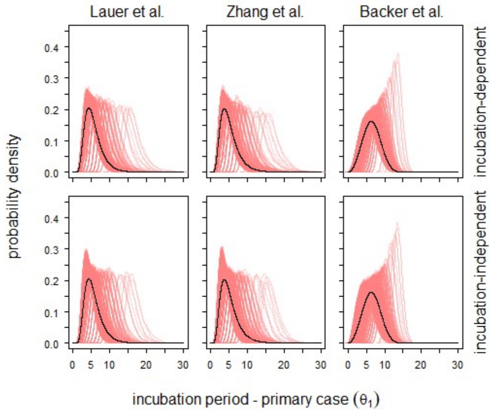
Fig. S3 Overlaid posterior distributions for the incubation period of the primary case ( \theta_1 ) of each case pair in the post-lockdown period. Black lines show the incubation period prior for each analysis.
