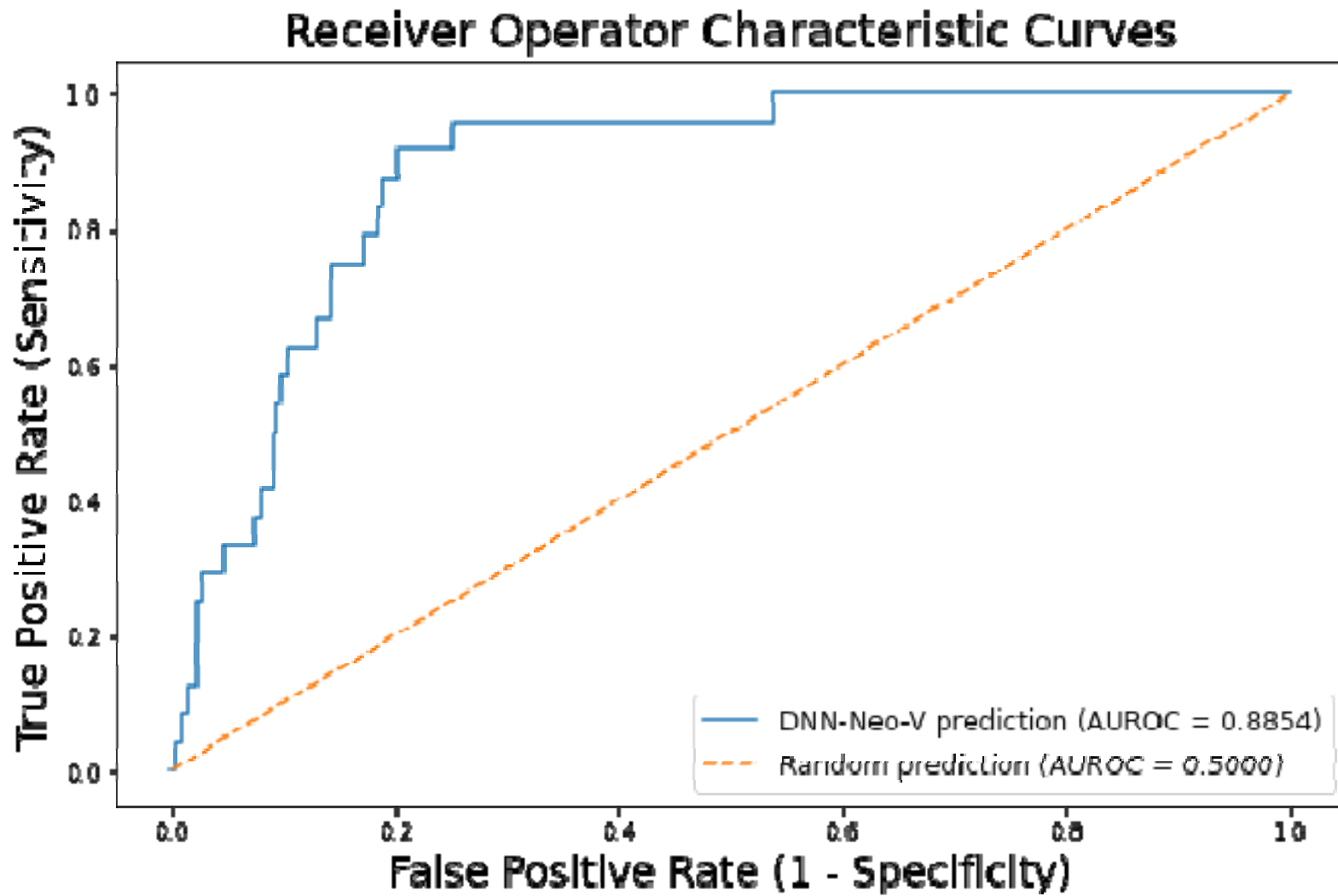
Figure 2. Receiver Operating Curve for Deep-Neo-V with AUROC
