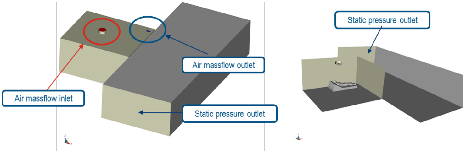
Supplementary Fig. S6. Boundary conditions of the simulation and ICU room geometry showing the position of the ventilation inlet and outlet
