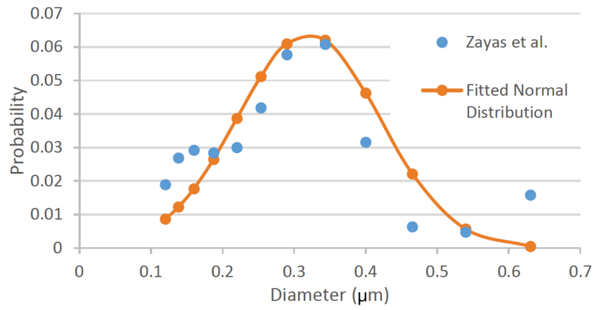
Supplementary Fig. S3. Particle size distribution used in the simulation (Zayas et al., 2012)
