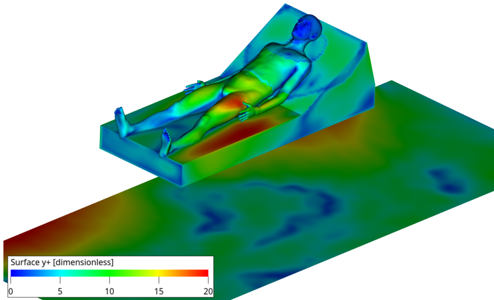
Supplementary Fig. S13. Y^+ map around the patient
