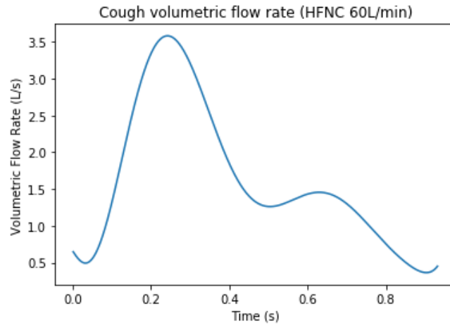
Supplementary Fig. S2. Quantitative result from Schlieren images of a volunteer's cough with HFNC at 60L/min after polynomial interpolation. The cough volumetric flow rate is estimated through PIV analysis, extrapolation and integration of all video frames. It is similar to the one used in the model: identical shape with two peaks, comparable volume of exhaled air.
