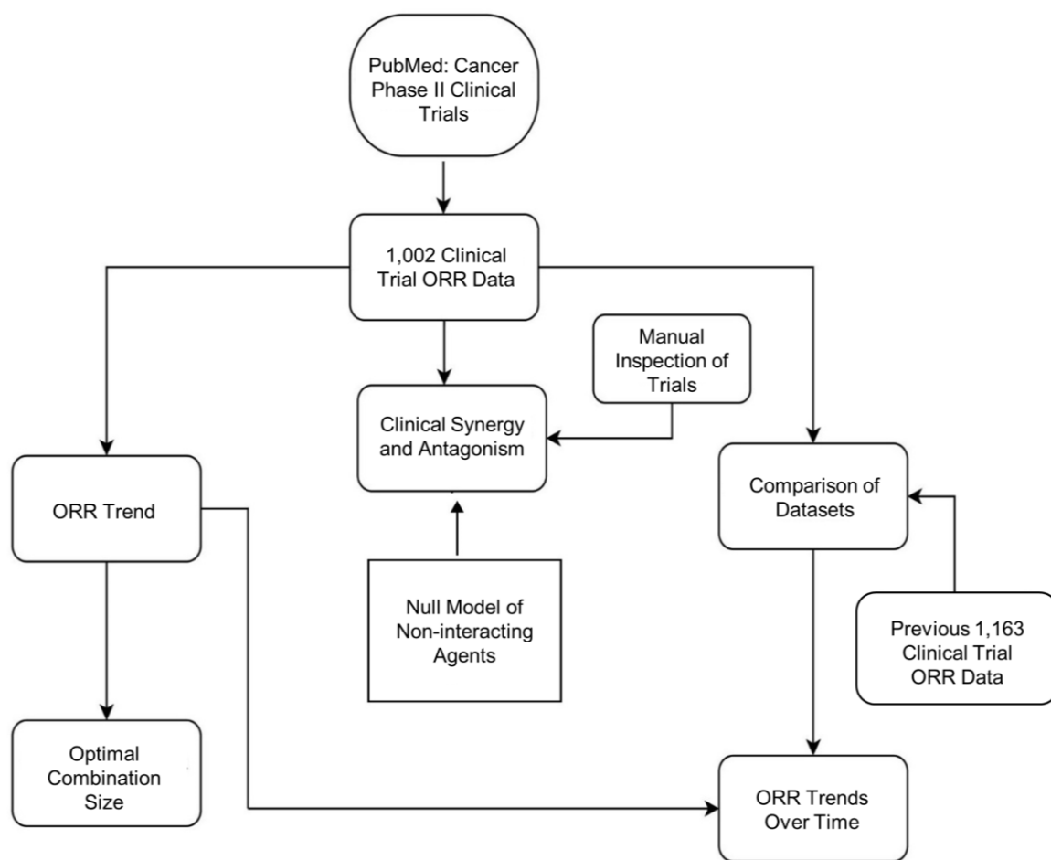
Figure 1: Study design and workflow.
