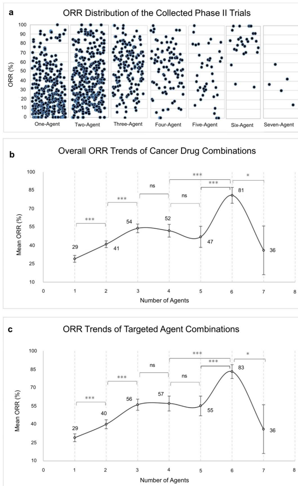
Figure 2: ORR increases with increasing number of agents in combination.
