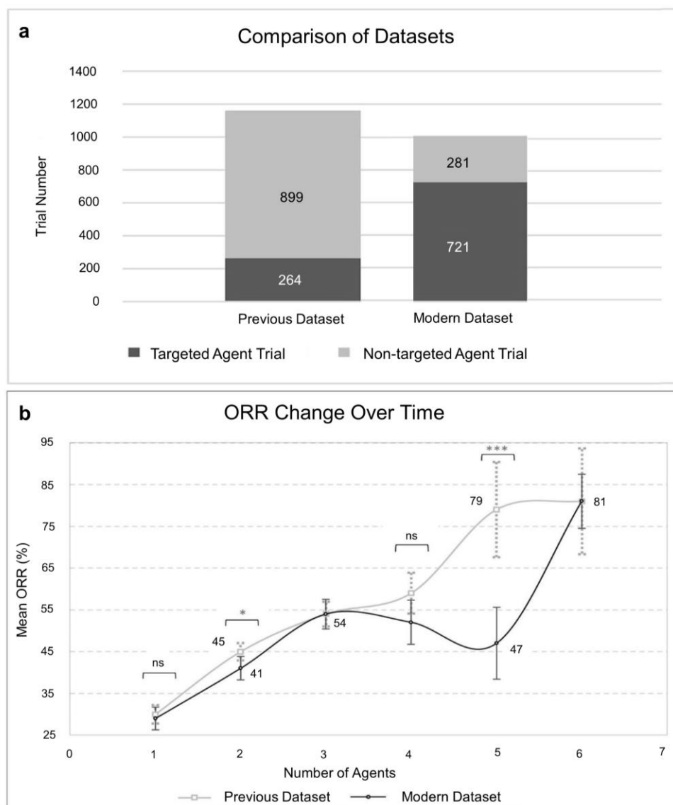
Figure 3: Increasing the number of targeted agents does not increase ORR.
