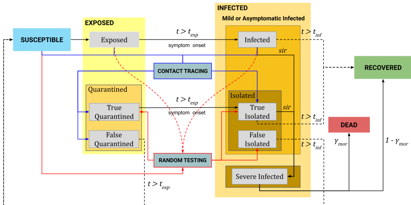
Fig. 2. The statechart of the particle-based SEIR epidemic simulator.
