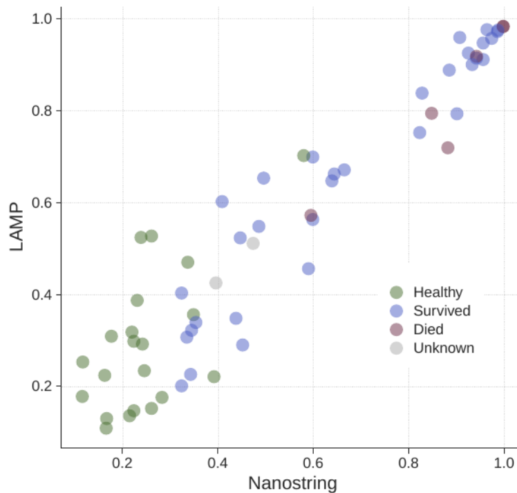
Supplementary Figure 2. Correlation of the 6-mRNA classifier scores using rapid qRT-LAMP panel and NanoString nCounter gold standard shows excellent agreement (Pearson R = 0.95) across n=61 clinical samples.
