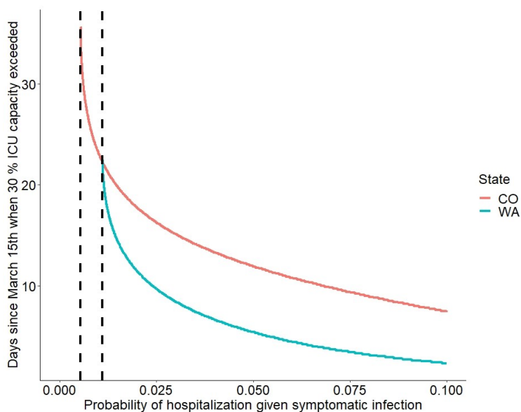
Figure 3: Dotted vertical lines represent asymptotes – the probability beyond which the ICU bed cap would not be exceeded from March 15th – May 18th . For both models E_0 = 30 \cdot I_0 , H_0 = 10 \cdot h_0 , and p = 0.86 and \chi = 1 .
