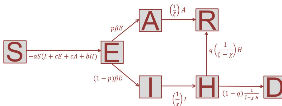
Figure 1: A compartment diagram depicting the system of ordinary differential equations used in this study. See Tables S5 and S6 for variable and parameter definitions.
