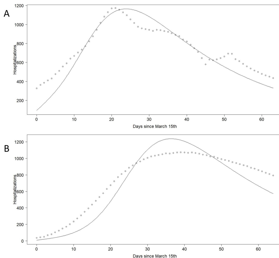
Figure 5: (A) Points are counts of hospitalized COVID-19 patients in all WA hospitals by day, corrected for underreporting by hospitals. Curve is H(t) function output from SEAHIRD model multiplied by the probability of hospitalization given symptomatic infection, which was numerically estimated as 0.0286. (B) Points are counts of hospitalized COVID-19 patients in all CO hospitals by day, corrected for underreporting by hospitals. Curve is H(t) function output from SEAHIRD model multiplied by the probability of hospitalization given symptomatic infection, which was estimated to be about 0.0234. For both (A) and (B), SEAHIRD initial conditions included E_0 = 30 \cdot I_0 and H_0 = 10 \cdot h_0 while p = 0.86 and \chi = 1 .
