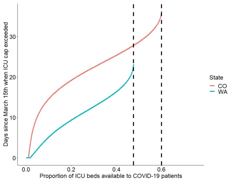
Figure 4: Dotted vertical lines represent asymptotes – proportion of ICU bed availability beyond which the ICU bed cap would not be exceeded from March 15th – May 18th . For both models E_0 = 30 \cdot I_0 , H_0 = 10 \cdot h_0 , and p = 0.86 and \chi = 1 .
