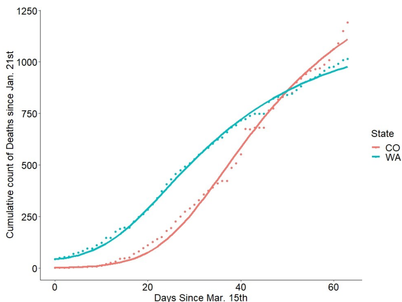
Figure 2: Points are raw counts of deaths due to COVID-19 since Jan. 21st - colored by the state in which the deaths occurred - and the lines are the SEAHIRD model fits to these points. Best fit parameters were \alpha = 7.954e-07 and S_0 = 4.893e+05 for the WA SEAHIRD model and \alpha = 5.410e-07 and S_0 = 7.477e+05 for the CO SEAHIRD model. For both models E_0 = 30 * I_0 , H_0 = 10 * h_0 , and p = 0.86 and \chi = 1 .
