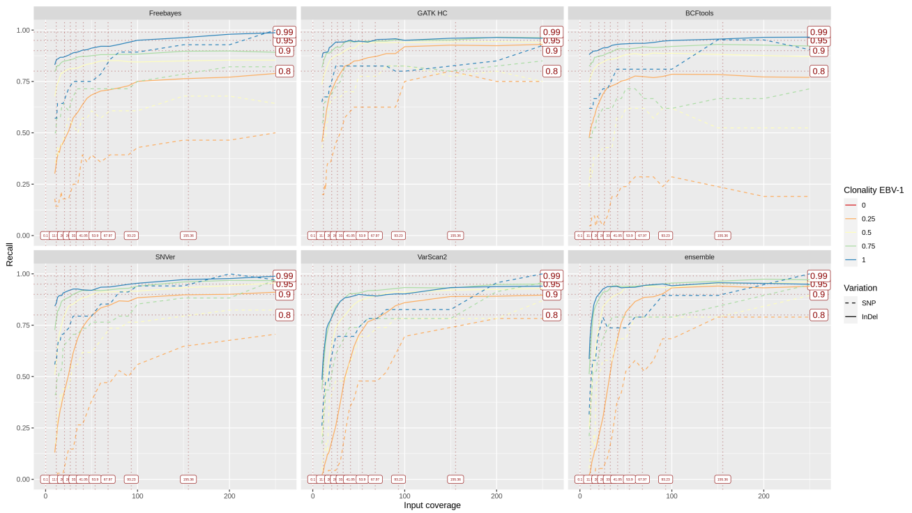
Supplementary Figure S7b: Performance of Freebayes, GATK HC, BCFtools, SNVer, VarScan2 against the synthetic read libraries. The ensemble plot shows the intersection of GATK HC, SNVer and VarScan2. The reads were mapped using BWA mem against AG876. The clonality (blue to red gradient) is referred as the percentage of EBV-1 reads in the libraries. The vertical axis is the recall, namely, the variant counts of a caller in a given dataset over the size of the union of all variants found in all datasets by this caller. The vertical dashed lines are the decile of the mean read depths of EBV reads in the SHCS samples.
