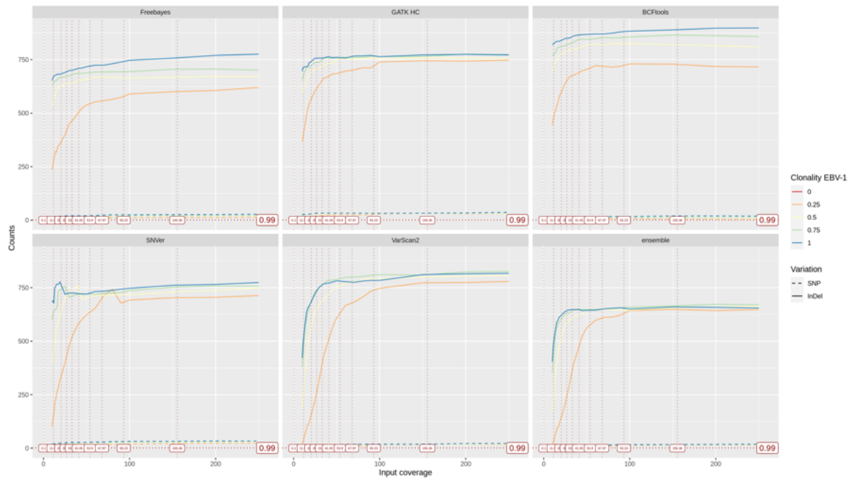
Supplementary Figure S7c: Raw variant counts by GATK HC, BCFtools, SNVer, VarScan2 against the synthetic read libraries. The reads were mapped using BWA mem against AG876. The noticeable artifact observed in SNVer did not affect the result of the ensemble, let alone the result of the other callers.
