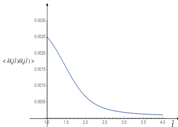
Figure 18: Correlation function \langle (\delta I_h(t))^2 \rangle for Italy, first wave of infection by SARS-CoV-2. This correlation function is the solution of second equation of the system (59). Having chosen our reference state I_{hRS} = C_h , we get a typical correlation function for random fluctuations at equilibrium.
