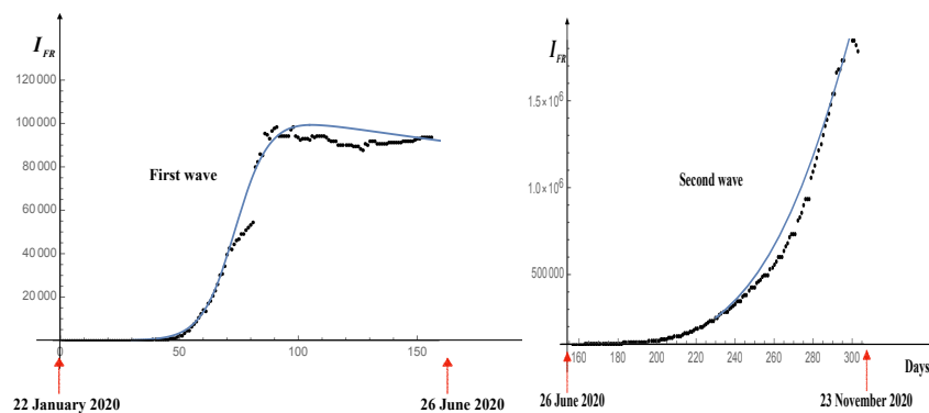
Figure 24: Comparison between the theoretical predictions (blue line) and real data (black dots) for France during the first wave of Coronavirus. The values of the parameters are; \tilde{\alpha} = 0.145 \text{ day}^{-1} , \beta = 0.5 \text{ day}^{-2} , K = 110000 , and t_L = 53 days, respectively.
