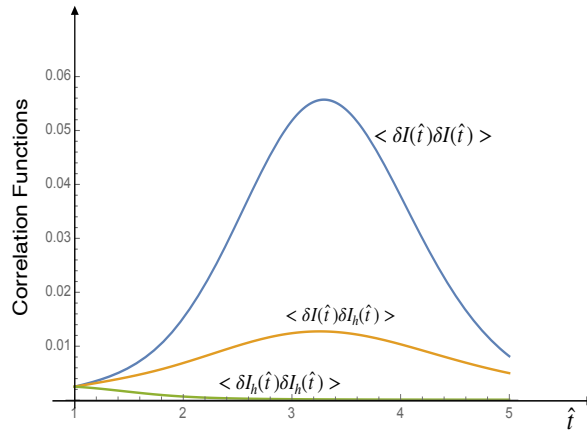
Figure 19: Correlation functions \langle \delta I(t)\delta I(t) \rangle , \langle \delta I_h(t)\delta I_h(t) \rangle , and \langle \delta I(t)\delta I_h(t) \rangle . These three correlation functions are obtained by solving numerically system (59).
