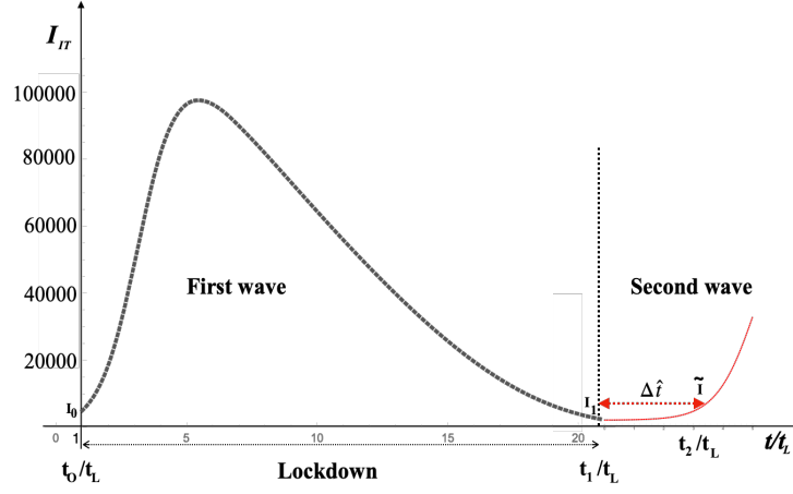
Figure 2: Schematic representation of the second wave of SARS-CoV-2 infection. The Lockdown measures are applied during the period \hat{t}_0 - \hat{t}_1 . At the end of the confinement measures, the number of infectious dropped to I_1 . During the time interval \Delta \hat{t} = \hat{t}_2 - \hat{t}_1 , the lockdown measures are not applied and the infection by SARS-CoV-2 (starts growing again (second wave of Coronavirus infection) until the preset value \tilde{I} is reached, which corresponds to I(\hat{t}_2) . During the whole time interval \Delta \hat{t} , the number of infectious individuals still stay below a set threshold \tilde{I} if I_1 satisfies condition (25).
