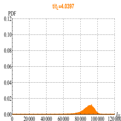
Figure 11: Probability density function (PDF), solution of Eq. (36). Screenshot at time \hat{t} = 4.0397 .
