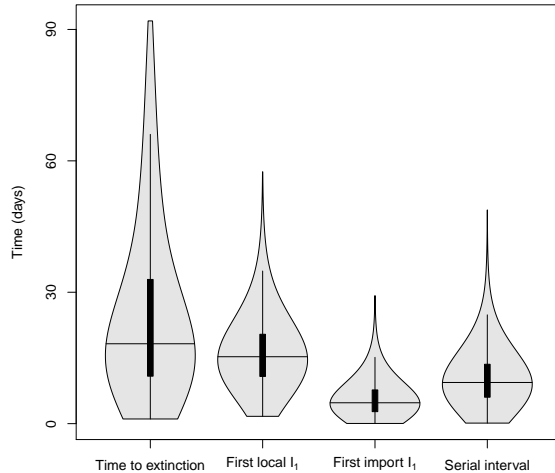
Figure ES.2: Time to extinction of the disease, first detected locally infected individual, first detected imported case, and serial interval. Base case simulation with S(0) = 142,906 (population of Prince Edward Island), L_1(0) = 1 and all other states equal to 0. Horizontal lines indicate the median value. Black rectangles are the inter-quartile range. Here, \mathcal{R}_t = 0.8 .
