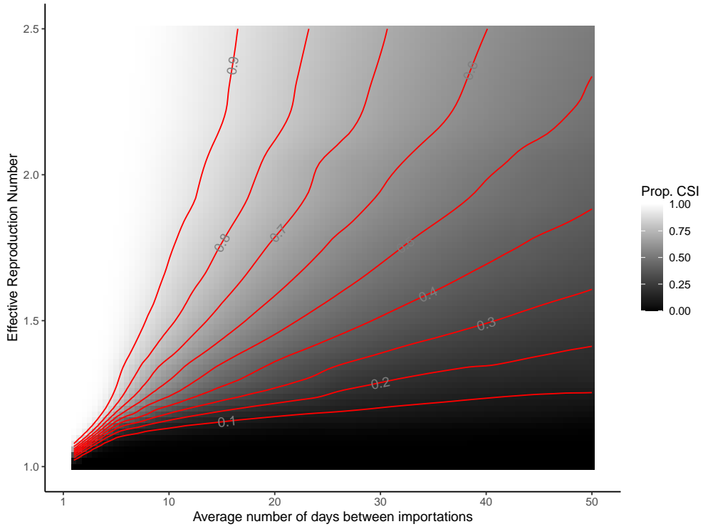
Figure ES.3: Proportion of critical successful importations (CSI) in a 3 month period for different values of the average number of days between two importations and \mathcal{R}_t , an indicator of NPI efficacy.
