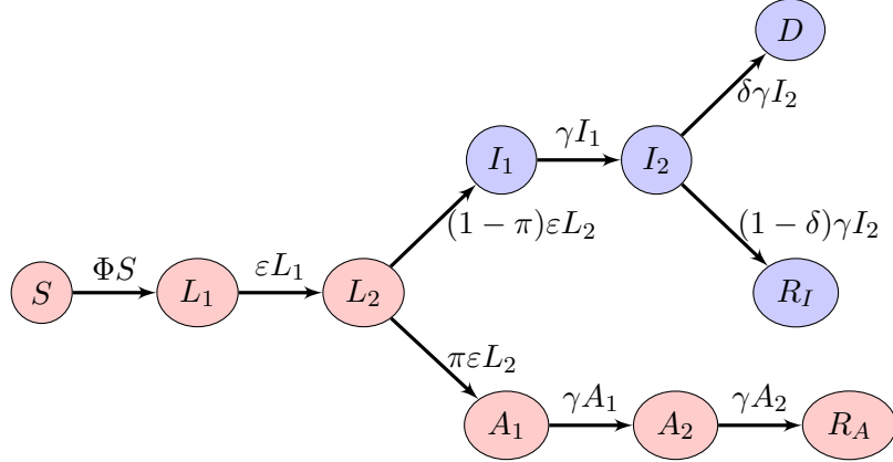
Figure ES.1: Flow diagram of the SL_1L_2I_1I_2A_1A_2R_I R_A D model. \Phi = \beta(I_1 + I_2 + \xi(A_1 + A_2) + \eta L_2) is the force of infection. Blue compartments are observable (detected), with I_1 and I_2 usually indistinguishable and observed as I_1 + I_2 .
