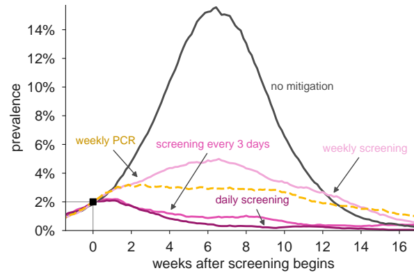
Figure 5: Impact of olfactory dysfunction screening on an ongoing viral outbreak Examples of the impact of screening programs based on olfactory dysfunction on controlling an ongoing outbreak. Viral spread in fully-mixed community of 20,000 individuals was allowed to proceed until prevalence reached 2%, at which point olfactory dysfunction (OD) screening was initiated either daily (dark red), every three days (red), or weekly (pink). For comparison, weekly RT-PCR testing with a one-day turnaround is shown (dashed yellow line). Olfactory dysfunction is modeled to be present in 75% of infected individuals, last 7 days, and to begin one day after viral levels reach \sim 1000 virions/ml. We consider 80% participation in testing. Scenario without mitigation is shown for comparison (black).
