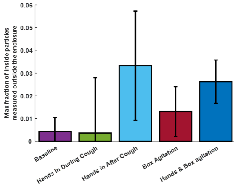
Figure S4: Different results of the agitation experiments with error bars representing standard deviation between 3 trials. The 2-layer furniture wrap and Steri-Drape were used for these experiments, with hands covered in nitrile gloves. Baseline is the 2-layer covered enclosure with no hands or jostling. No statistical difference was found with one-way ANOVA. Jostling and inserting/removing hands in the box will not lead to large increases in particle concentrations outside of the box.
