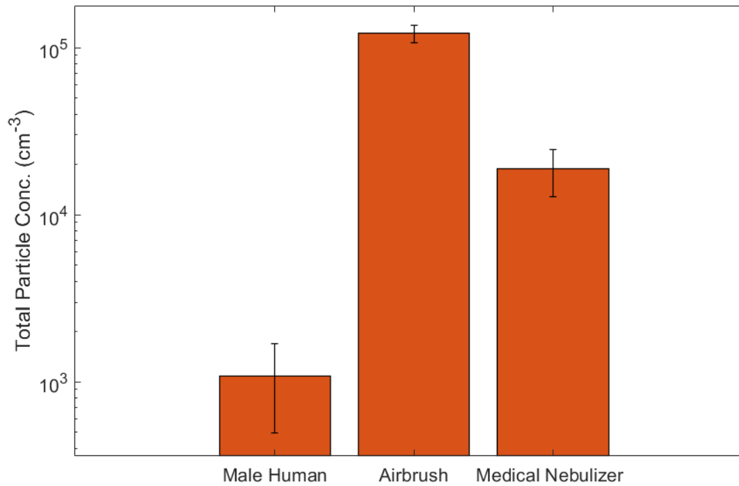
Figure S3: Comparison of total particle concentration generated from real and simulated coughs. The average male human cough (Yang et. al, 2007) compared with the simulated Paasche airbrush cough and an extended burst from the Omron medical nebulizer. The medical nebulizer and airbrush means are derived from the peak concentration achieved within the uncovered enclosure.
