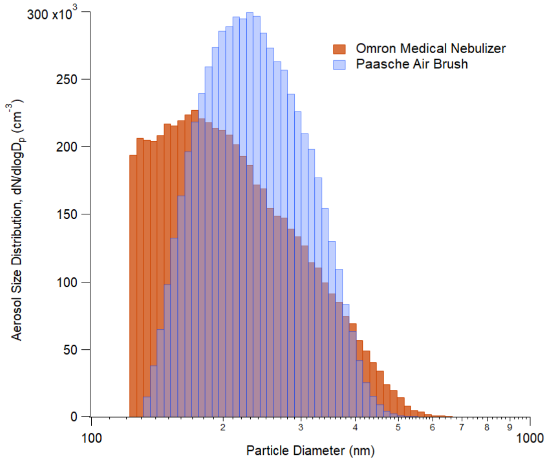
Figure S1: Number size distributions of particles between 0.12 \mu\text{m} and 0.6 \mu\text{m} generated by the Paasche airbrush (blue) and Omron medical nebulizer (orange) measured with the scanning mobility particle sizer (SMPS). Particles below 120 nm were not measured to shorten measuring time to limit the impact of the initial rapid particle decay. It is also presumed that viral particles would not be able to be present in particles below this size. The airbrush has a mode at 0.23 \mu\text{m} and the medical nebulizer at 0.17 \mu\text{m} .
