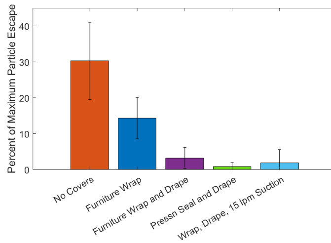
Figure 2: Ratio of the maximum aerosol mass concentration measured inside vs. measured outside the enclosure for particles larger than 0.1 microns when various types of one-layer of plastic covering with or without an added Steri-Drape layer were placed over the front and side holes in the enclosure.
