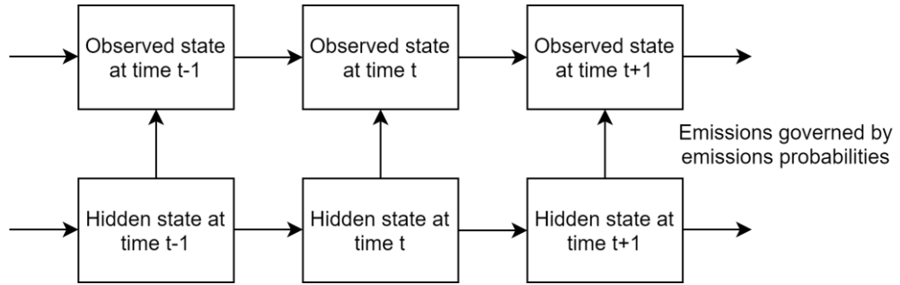
Figure S11: The structure of a Hidden Markov Model.
