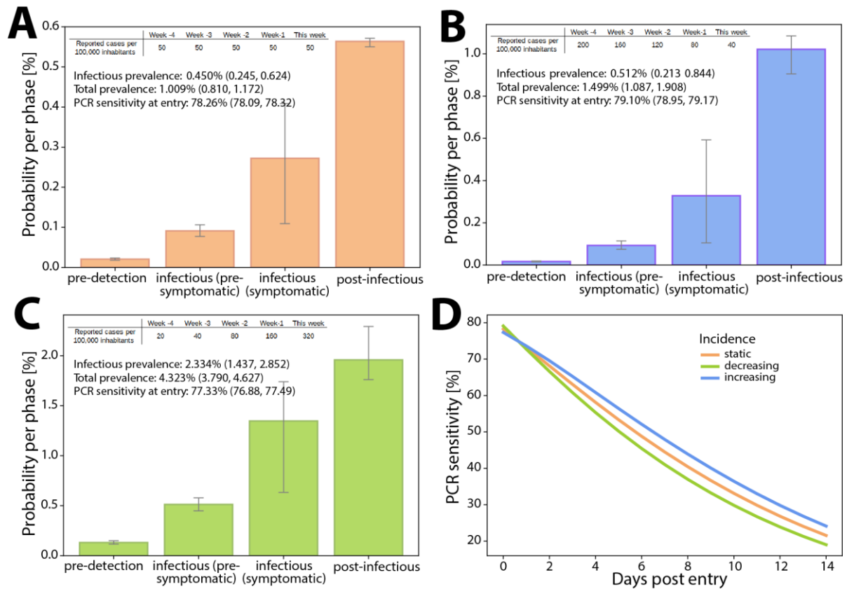
Figure 4: Pre-entry risk calculation for incoming travellers. A. Prevalence estimation for travellers entering from a country with a stable incidence (50 cases/100,000/week for the last 5 weeks), B. a declining incidence (200, 160, 120, 80, 40 cases/100,000/week for the last five weeks) and C. a rising incidence (20, 40, 80, 160, 320 cases/100,000/week for the last five weeks). D. Time-dependent PCR sensitivities in the respective cohorts of travellers in the days post-entry.
