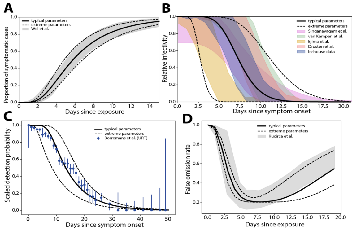
Figure 2: Model validation. Published- and data-derived SARS-CoV2 intra-patient dynamics (shaded areas), as well as model-predicted dynamics with default parameters (lines). A. Duration of incubation. The cumulative time-to-symptom onset from a meta-analysis of fifty six studies is shown (grey shaded areas) 53 , together with the model-predicted time-to-symptom onset (solid line: typical dynamics, dashed lines: upper and lower extremes). B. Relative infectiousness after symptom onset/peak viral load extracted from Singanayagam et al. and van Kampen et al. 55,56 , deduced from in-house data (Supplementary Note 3) and derived from viral load kinetics reported by Ejima et al. 54 59 are shown as shaded areas, whereas model-predicted infectiousness profiles are depicted by lines (solid line: typical dynamics, dashed lines: lower and upper extremes). C. Time-dependent PCR sensitivity after symptom onset reported by Borremans et al. 57 (error bars) together with model simulated PCR sensitivity using default parameters (solid line: typical dynamics, dashed lines: lower and upper extremes). D. Time-dependent false omission rate as reported by Kucirca et al. 58 (shaded area). Solid- and dashed lines show model simulations with typical- and upper/lower extreme parameters. Details on the parameter fitting procedure and analysis of infectivity profiles are provided in Supplementary Note 2-3.
