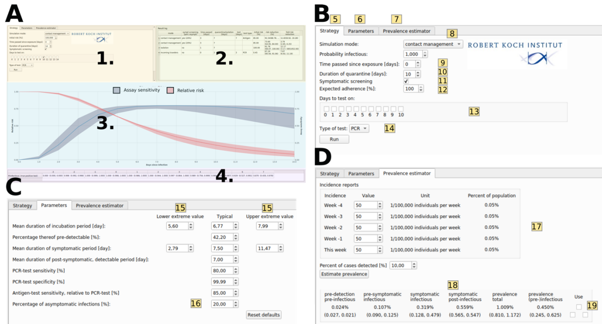
Figure 3. Screenshot of CovidStrategyCalculator. A. The main window consists of four components: user input (1), a result log (2), time course trajectories (3) and test efficacy reports (4). Reported results include the pre-procedure risk (prevalence), post-procedure risk (residual risk) and fold risk reduction. B. Zoom-in on the strategy-related user input. C. Model parameter input tab. D. Prevalence estimator input tab.
