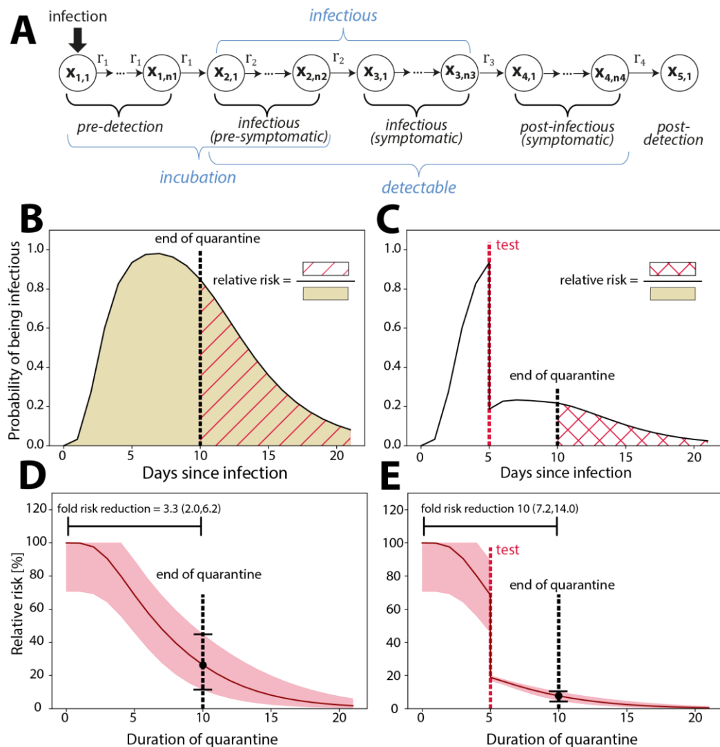
Figure 1: Simulation of Quarantine and testing strategies. A : Model structure. B : Model simulated probability of infectiousness. The shaded area indicates the risk emanating from an infected individual. If a quarantine was imposed until day 10 (dashed black vertical line), the risk of transmission would relate to the red-dashed area. Hence the risk reduction denotes the risk after the quarantine divided by the risk without quarantine. C : Model simulated probability of infectiousness when a test (dashed red vertical line) was performed at day 5. If the test was positive, the person would go into isolation, thus not posing a risk, whereas there is a residual risk that the person is infectious, if the test is negative (false negative). The risk after a 10 day quarantine (dashed black vertical line) with a test at day 5 is indicated by the red crossed area. D : Relative risk corresponding to a pure quarantine as indicated in panel B. E : Relative risk corresponding to a testing and quarantine scenario as indicated in panel C.
