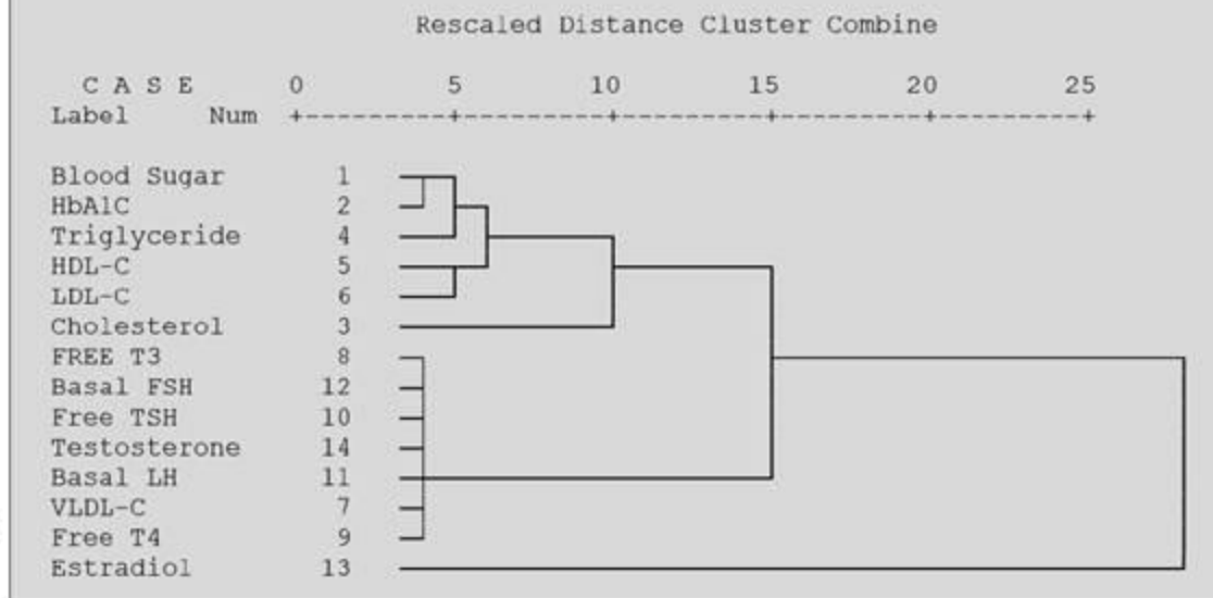
Fig. 1.b. Hierarchical representation of the diagnostic parameters for the two PCOS Phenotypes
