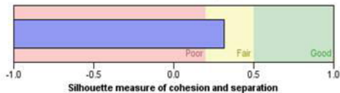
Fig. 1. a. Model summary of the two-step cluster analysis with a graph of the quality of clusters
