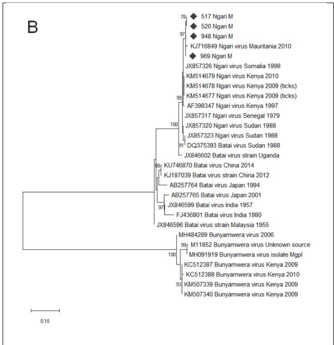
Fig. 2 Phylogenetic tree of sequences of Ngari virus-derived A) fragments of the S segment (346 bp) and B) fragments of the M segment (330 bp) of Bunyamwera virus and Batai virus compared with those of isolates obtained from ixodid ticks in Guinea in 2018 (filled diamonds). The trees were constructed by using the maximum-likelihood method (1,000 bootstrap replications) and the Tamura 3-parameter model. A discrete gamma distribution was used to model evolutionary rate differences among the sites. The trees are drawn to scale, with branch lengths corresponding to the number of substitutions per site.
