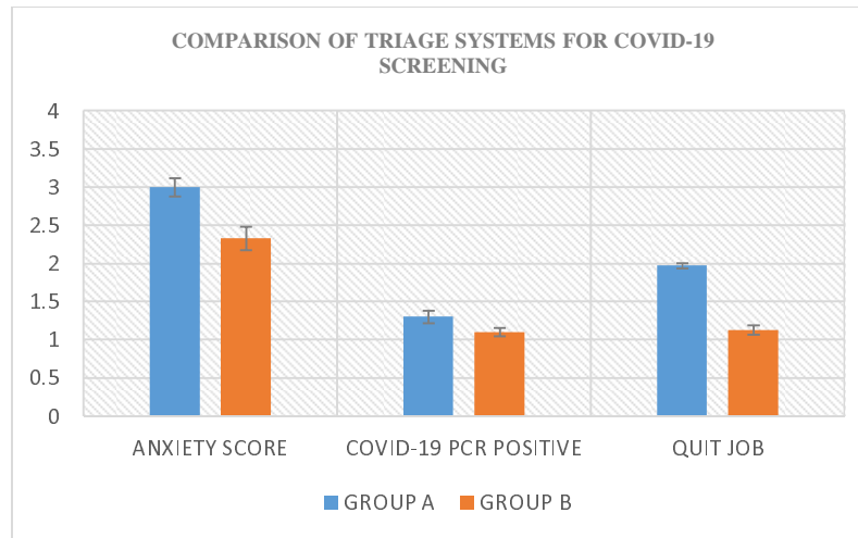
Graph-1: Comparison of Triage Systems for COVID-19 Screening
