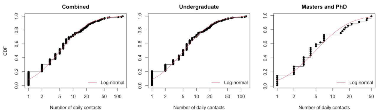
Fig. 2: Cumulative distribution functions for number of daily social contacts (outside of society and sports clubs) for all students, undergraduates and postgraduates. Black dots and lines depict the empirical data. The red solid line corresponds to the best-fit lognormal distribution.
