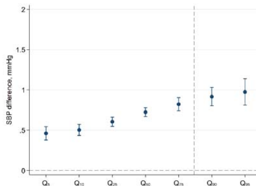
Figure 3. Associations between body mass index and systolic blood pressure quantiles (mmHg) across adulthood ( \geq 25 years, from repeated cross-sectional data, left panel), and midlife (43-46 years, from birth cohort data, right panel). Note: SBP values adjusted for use of antihypertensive medication (by adding a constant of 10mmHg for those using antihypertensive medication; estimates are adjusted for sex and education attainment.
