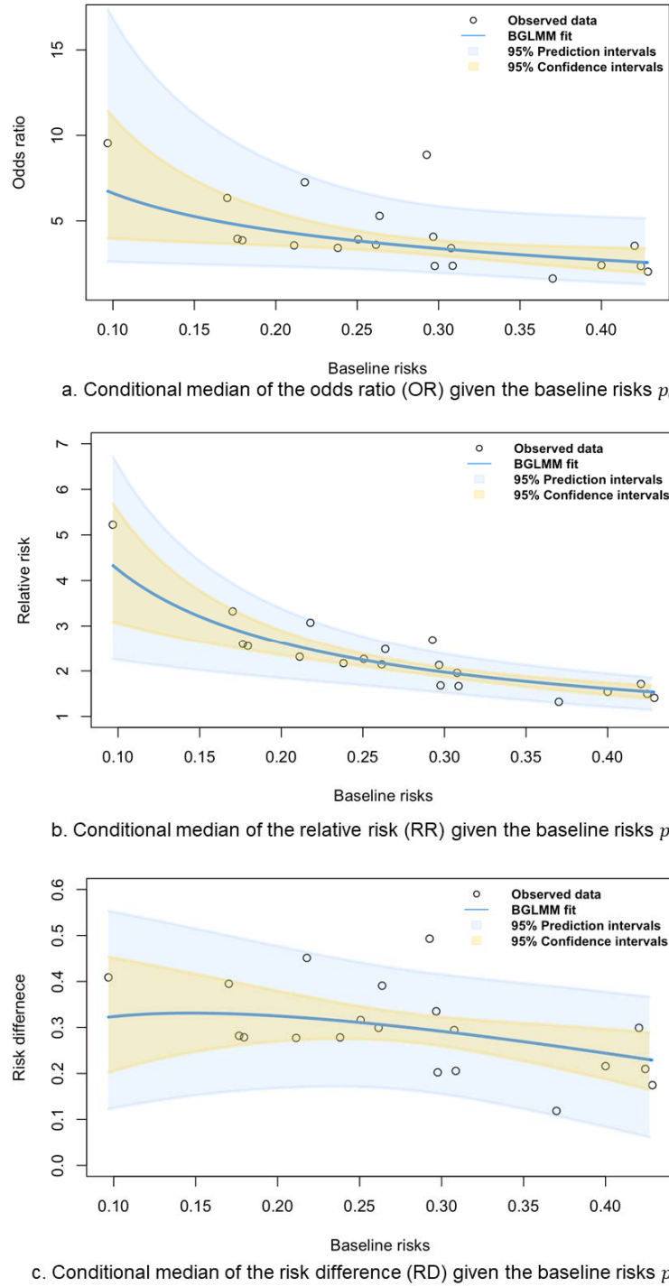
Figure 2: Plot of the observed OR, RR, and RD versus the nonlinear fit from BGLMM with varying levels of baseline risks; BGLMM: bivariate generalized linear mixed-effects model; OR: odds ratio; RD, risk difference; RD, relative risk.
