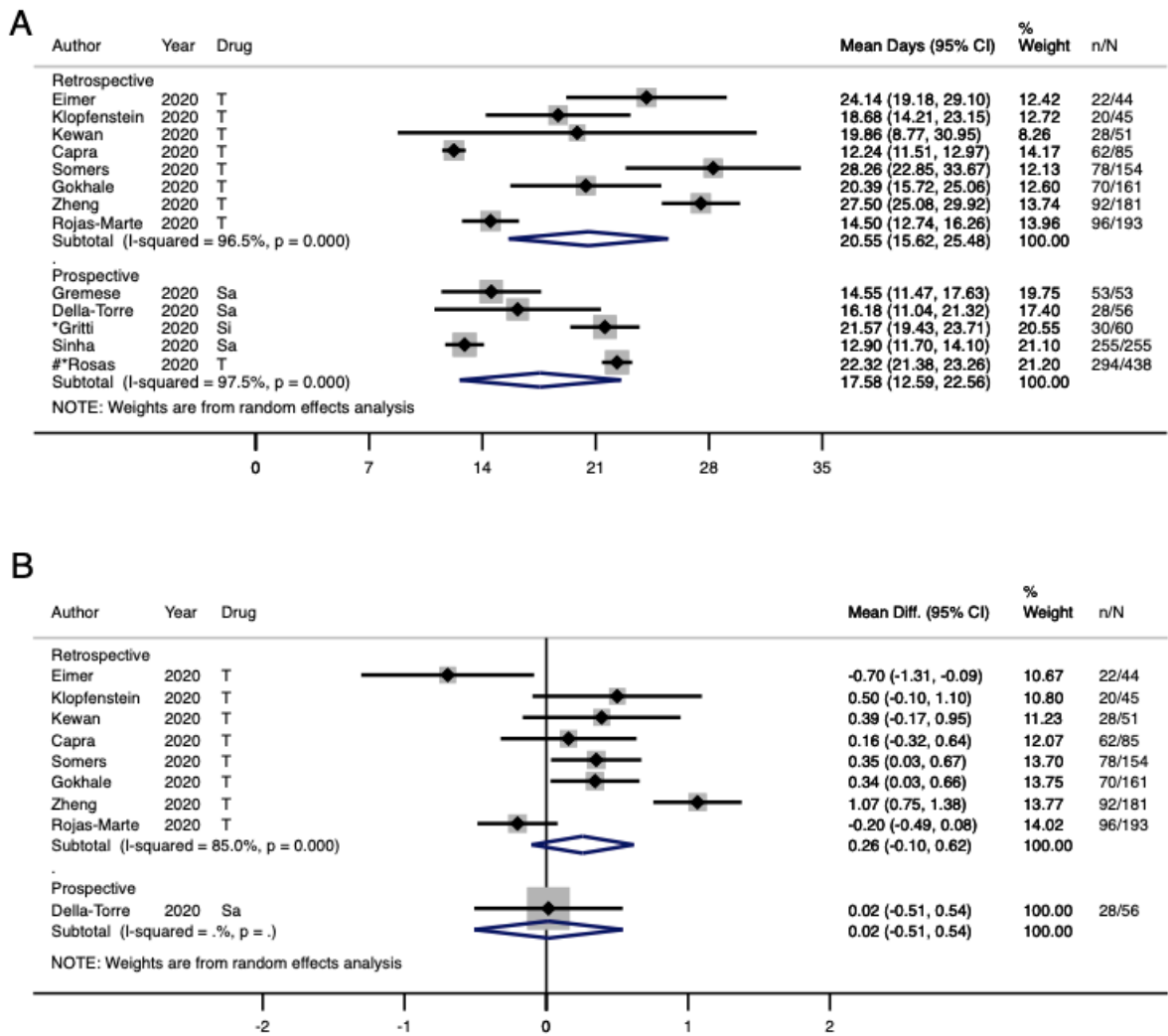
Supplementary Figure 5 – All studies mean duration of hospitalisation (days) forest plot. A: Mean duration of hospital stay. B: Mean difference compared with controls in duration of hospital stay. Effect sizes and associated 95% confidence intervals presented for each study. Sample sizes given for patients receiving intervention (n) and total included in study (N). Summary estimates presented separately for prospective and retrospective studies. Drugs labelled where T = tocilizumab, S = sarilumab, Si = siltuximab.
