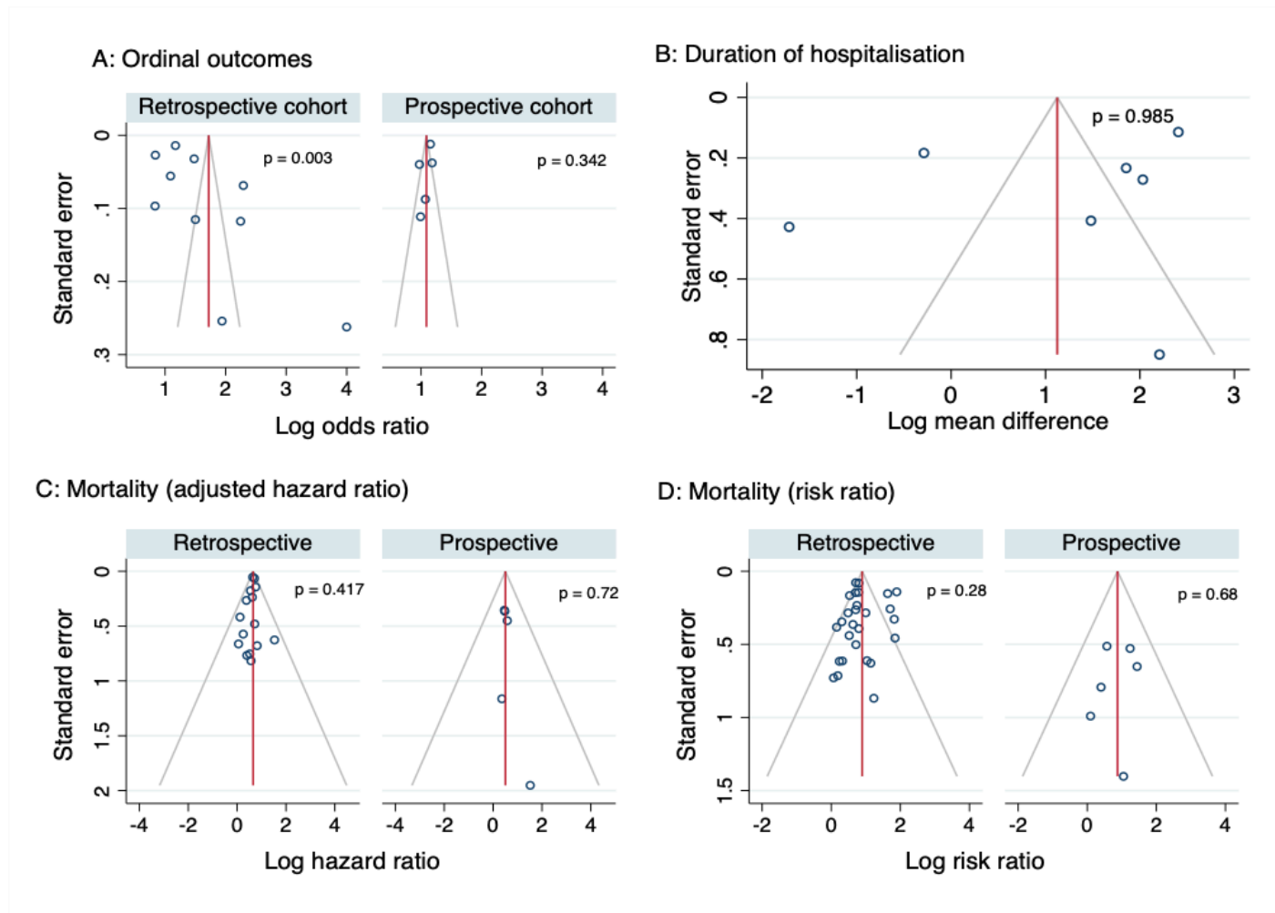
Supplementary Figure 8: Funnel plots for outcomes evaluated in meta-analysis of all agents. A: ordinal outcomes, B: duration of hospitalisation, C: mortality (adjusted hazard ratio), D: mortality (risk ratio). Funnel plots presented separately for retrospective and prospective studies were applicable. Publication bias assessed using Egger's test, and p values presented next to funnel plot.
