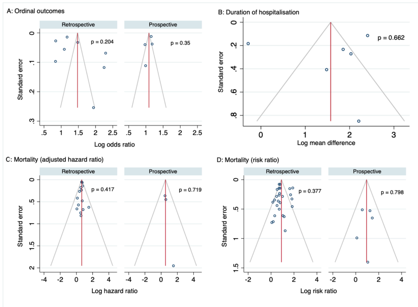
Supplementary Figure 3: Funnel plots for outcomes evaluated in tocilizumab meta-analysis. A: ordinal outcomes, B: duration of hospitalisation, C: mortality (adjusted hazard ratio), D: mortality (risk ratio). Funnel plots presented separately for retrospective and prospective studies were applicable. Publication bias assessed using Egger's test, and p values presented next to funnel plot.
