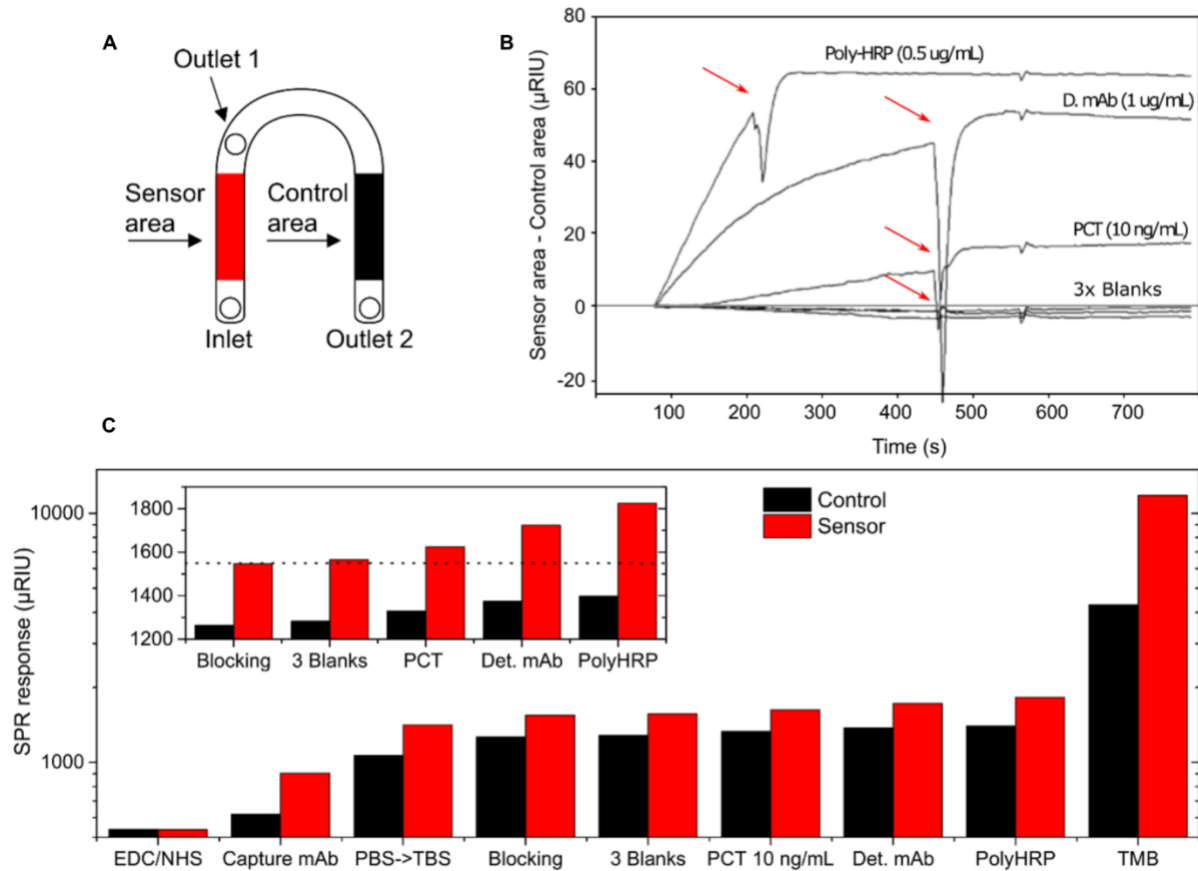
Figure S6. Validation of the PCT assay using SPR. Schematic representation of the SPR flow cell used in the study (A). Raw data obtained from the injection of blanks, PCT sample, detection mAb and Strep-pHRP. Red arrows indicate the transition between association and dissociation step (B). Combined data from sensor construction through pTMB precipitation. Inset presents closeup from blocking to Strep-pHRP steps (C).
