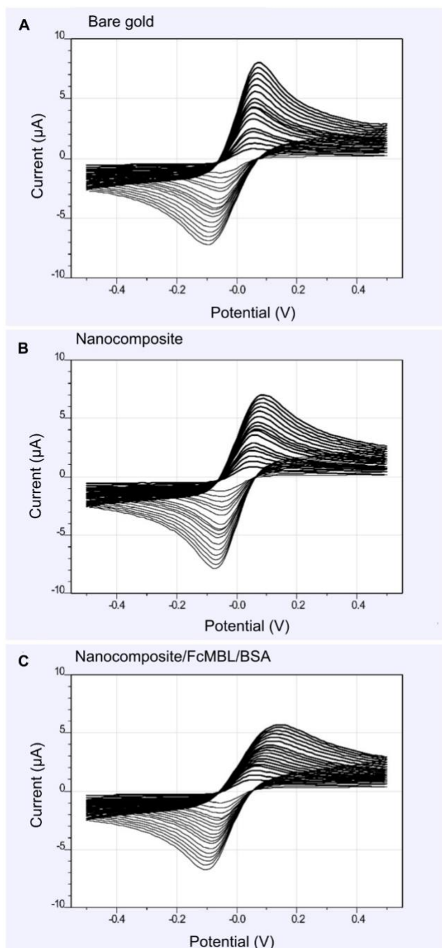
Figure S5. Oxidation and reduction current obtained in 5 mM ferri-/ferrocyanide using various scan rates between 0.01 V/s to 1 V/s on bare gold (A) BSA/rGOx/GA nanocomposite (B) and FcMBL functionalized nanocomposite after blocking with BSA (C).
