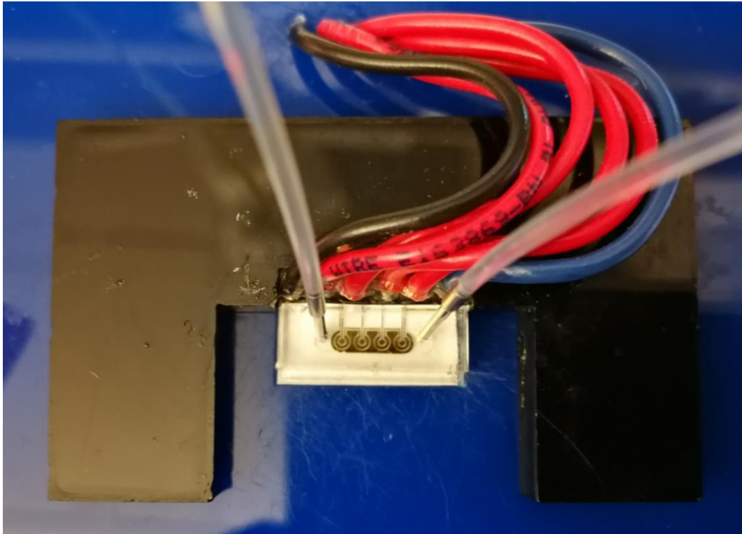
Figure S15. Picture of a microfluidic cell attached on the nanocomposite covered chip. Double sided adhesive was used to outline the channel and a PDMS block with an inlet and outlet holes is adhered on the top. Stainless steel connectors are inserted in the PDMS connecting the tubing to the microfluidic chamber.
