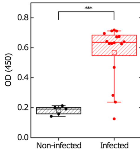
Figure S9. Box plot comparing PCT levels in infected and non-infected patient groups obtained with plate ELISA. Full circles represent the mean of measured PCT values, lines in a box represent median, 25 th and 75 th percentile, empty square is mean value, whiskers represent 10 th and 90 th percentile and *** represents p < 0.001 .
