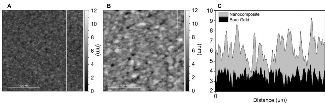
Figure S4. AFM analysis of bare gold and BSA/rGOx/GA nanocomposite. (A) Bare gold scan from which the profile was extracted. (B) BSA/rGOx/GA nanocomposite image from which the profile was extracted. (C) The extracted profiles of both samples.
