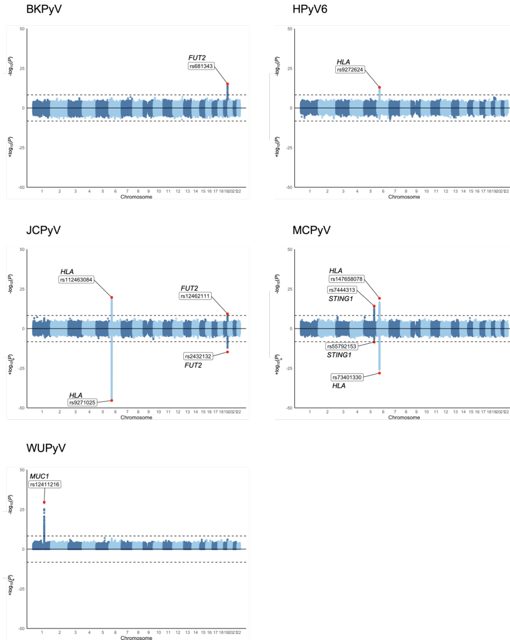
Figure 2. Chicago plots of genome-wide association results of the meta-analyses of antibody levels (top) and serostatus (bottom) against BKPvV, HPyV6, JCPyV, MCPyV and WUPyV. Chicago plots showing the significance of association of all SNPs across chromosomes 1 to 22. SNPs are plotted on the x-axis according to their physical position on each chromosome and the strength of the association with antibody levels is indicated on the y-axis (as -\log_{10} P -value for IgG response, and as +\log_{10} P -value for serostatus). The dashed line marks the Bonferroni-corrected genome-wide significance threshold of 5.6 \times 10^{-9} . For each locus, the SNP with the most significant association is plotted in red and labeled. Serostatus was not tested for WUPyV due to very high seroprevalence. Chromosome X is not shown since data were not available for all studies.
