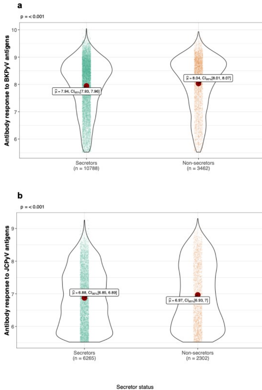
Figure 3. Serum immunoglobulin G (IgG) levels against BKPyV and JCPyV, by FUT2 genotype / secretor status. Violin plots show the log-transformed antibody levels (in MFI) against a) BKPyV and b) JCPyV. Antibody levels are categorized according to individuals, FUT2 secretor or non-secretor genotype. Red dots represent the mean. P-value based on t-test are shown.
