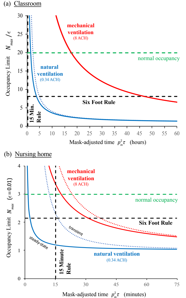
Fig. 3. The COVID-19 indoor safety guideline would limit the cumulative exposure time to lie beneath the curves shown. Evidently, the Six-Foot Rule becomes inadequate after a critical time, and the 15-Minute Rule above a critical occupancy. (a) Risk-adjusted occupancy, N_{max}/\epsilon , versus mask-adjusted time, p_m^2\tau , spent indoors with an infected person. We choose typical values appropriate for a school classroom: 20 persons share a room with an area of 900 square feet and a ceiling height of 12 feet ( A = 83.6 \text{ m}^2 , V = 301 \text{ m}^3 ). (b) Nursing home shared room with a maximum occupancy of three ( A = 22.3 \text{ m}^2 , V = 53.5 \text{ m}^3 ), and a risk tolerance of \epsilon = 0.01 chosen to reflect the vulnerability of the community. In both cases, curves deduced from the pseudo-steady formula, Eq. [5], are shown for both natural ventilation ( \lambda_a = 0.34/\text{h} ; blue curve) and mechanical ventilation ( \lambda_a = 8.0/\text{h} ; red curve). The transient occupancy (Eq.[13] in Methods) is shown with dotted curves. System parameters are C_q = 30 \text{ quanta/m}^3 , \lambda_v = 0.3/\text{h} , Q_b = 0.5 \text{ m}^3/\text{h} , \bar{r} = 0.5 \mu\text{m} , \bar{v}_s = 0.108 \text{ m/h} . We stress that in (a), the maximum occupancy is normalized by the risk tolerance \epsilon , the occupancy time by the squared mask penetration factor, p_m^2 ; thus, the deduction of concrete numbers for maximum occupancy N_{max} for a given time, or maximum occupancy time for a given N , requires an appropriate scale factor.
