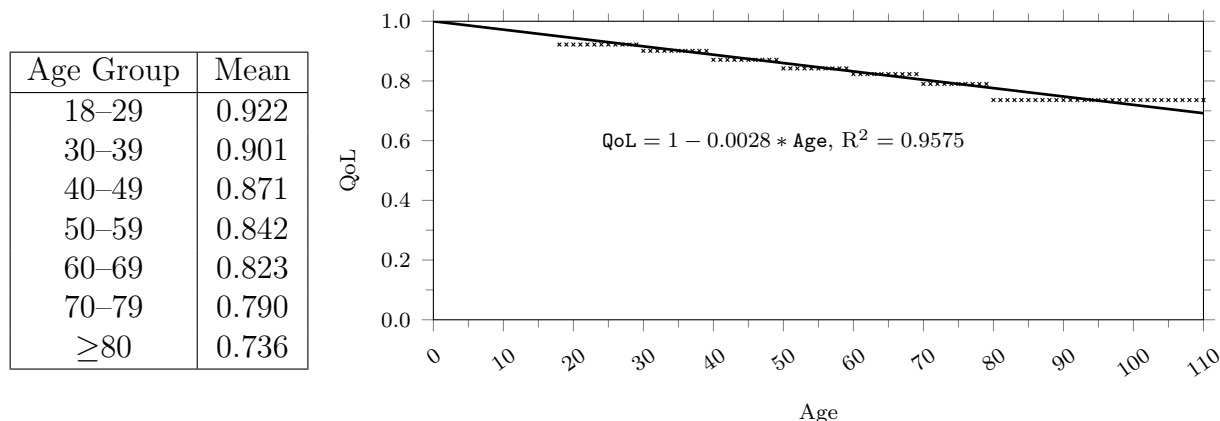
Figure 4: Age-dependent QoL, f_a(x) . The values extracted from ICER’s SMA final report [115] are replicated in the table on the left and are presented as crosses in the figure on the right. A linear line, with its intercept set to 1, is fitted with the data points.
