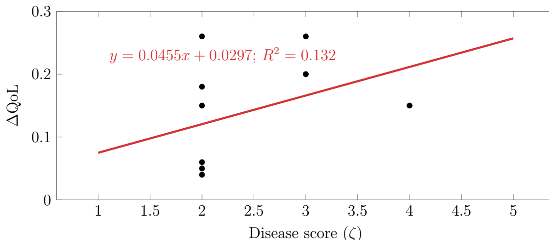
Figure 6: Scatter plot of \Delta QoL against disease score ( \zeta )
