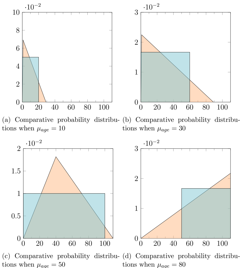
Figure A1: Age distributions given various mean ages, \mu_{age} . The red triangles represent the solutions obtained by our optimization program, while the blue rectangles represent the solutions given by an uniform distribution. The distributions from the optimization program have a wider base of support and avoid sharp changes in density.
