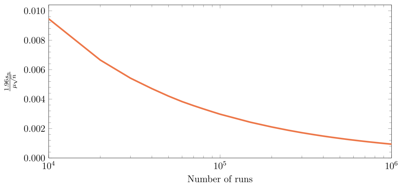
Figure A2: Plot of \frac{1.96s_n}{\mu\sqrt{n}} against the number of iterations of simulations of the cost.
