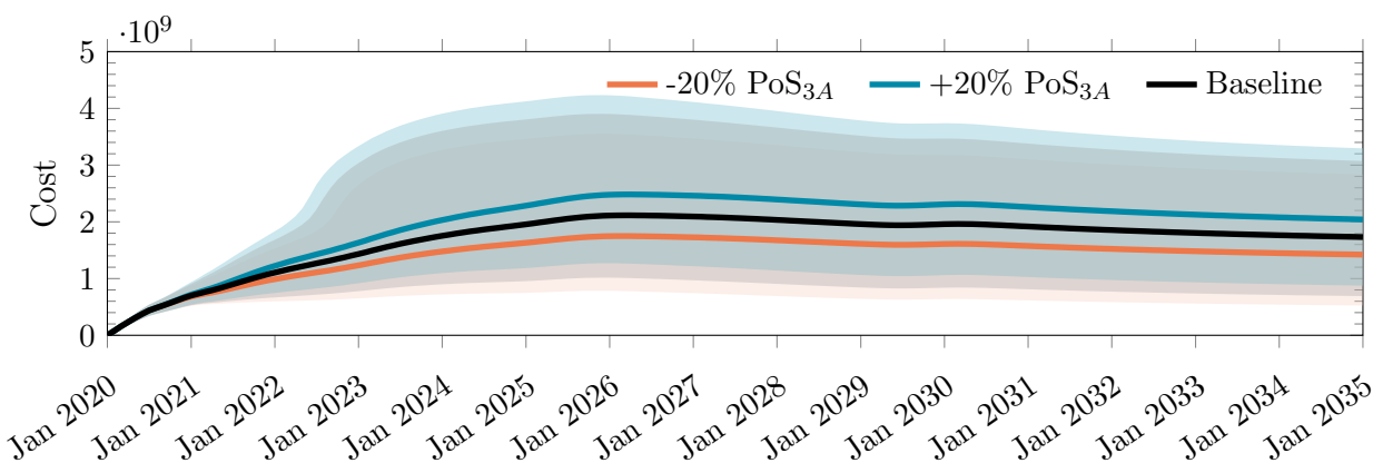
Figure A7: Impact on monthly cost of treating patients given a \pm 20\% change in the \text{PoS}_{3A} .
