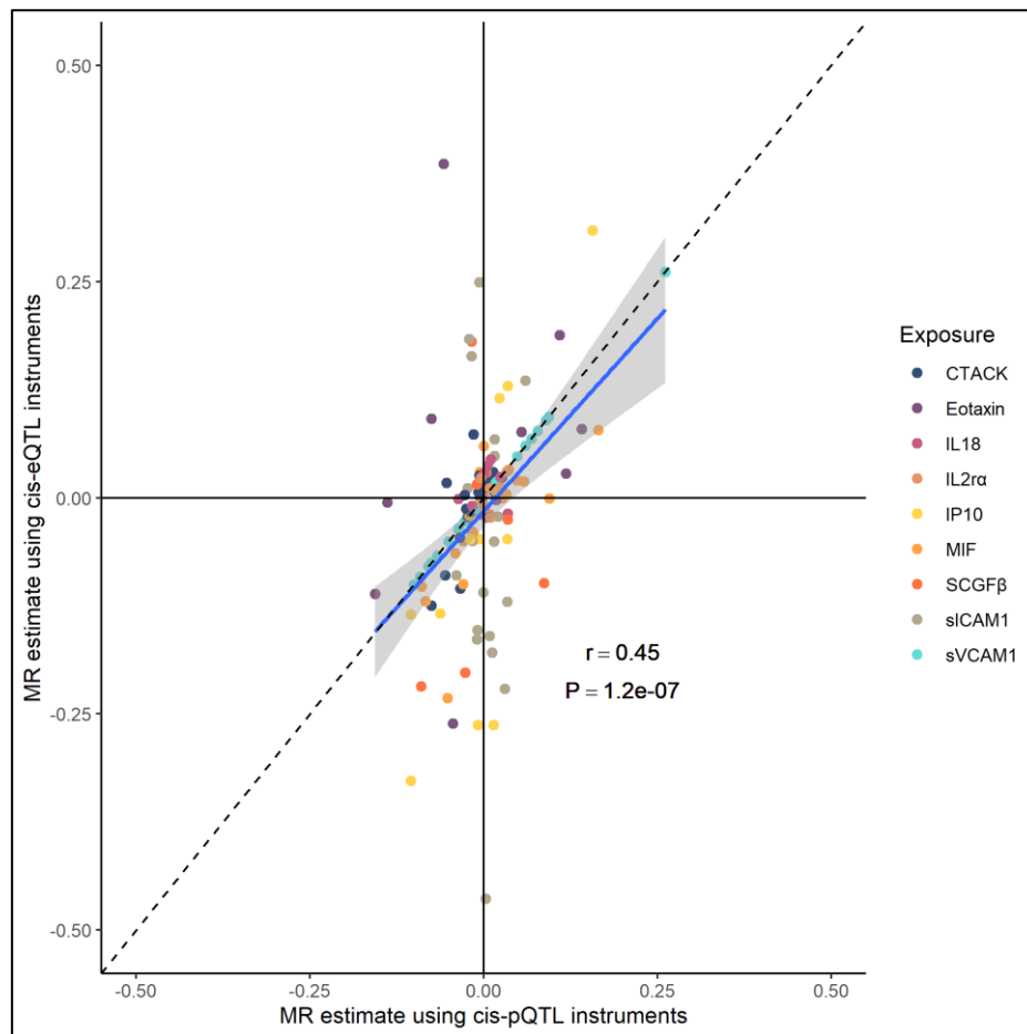
Figure 6. Scatter plot comparing Mendelian randomization (MR) estimates for the effects of genetically predicted cytokine levels on disease outcome traits when using the two different instrument selection criteria. The correlation between the MR estimates was quantified using Pearson's coefficient and a linear fit between effect estimates (blue line). x-axis: MR effect estimates using cis - protein quantitative trait loci instrument selection; y-axis: MR effect estimates using cis - expression quantitative trait loci instrument selection. r : correlation coefficient; P : p value.
