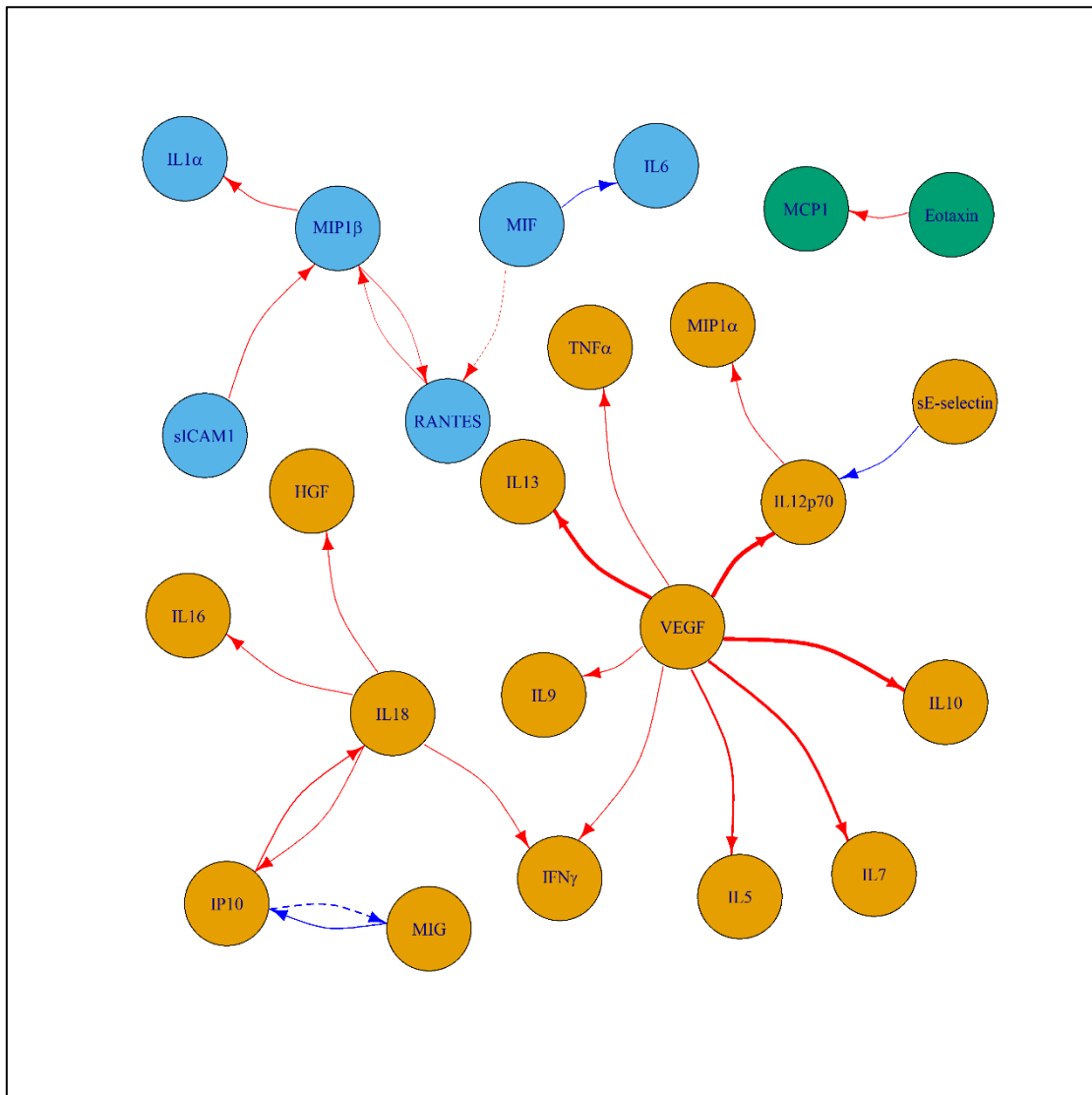
Figure 3. Mendelian randomization results of genetically predicted cytokine levels on levels of other circulating cytokines when considering cis - protein quantitative trait loci (solid lines) and cis -expression quantitative trait loci (dashed lines) instruments. The results are plotted only for effects with P < 0.0011 ( 0.05/\text{number of cytokines} ). Red and blue lines indicate positive and negative associations respectively. The thickness of the line represents the absolute value of the effect size. The colours of the cytokines represent separate cytokine groups based on the results.
