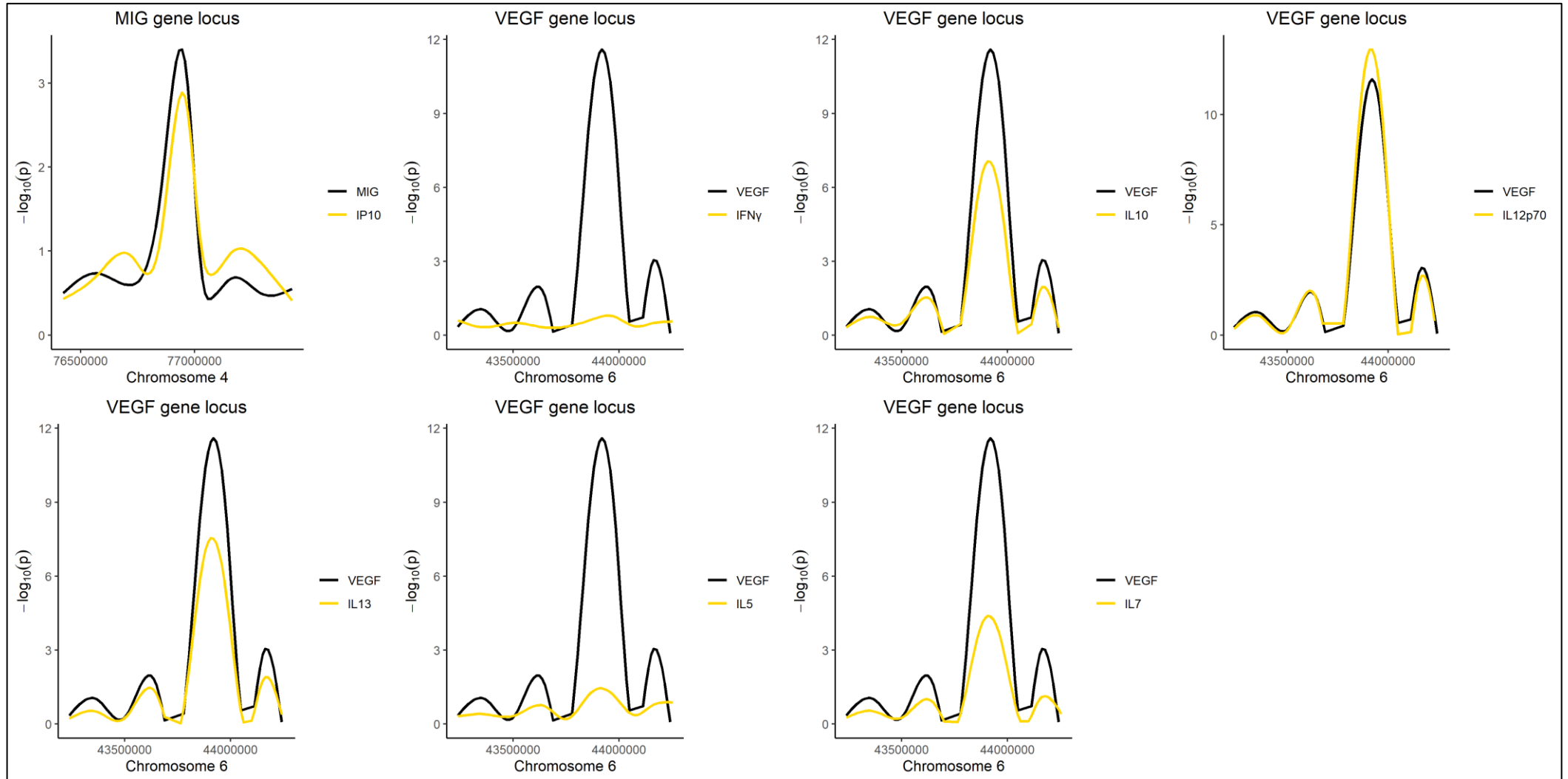
Figure 4. Colocalization for genome-wide association study summary statistics between selected cytokine pairs. Cytokine pairs that showed MR evidence for both causality ( P < 0.0011 ( 0.05/\text{number of cytokines} )) and colocalization (posterior probability > 0.9 ) are plotted, within \pm 500 kb of the gene locus of the exposure cytokine. The y-axis of -\log_{10}(p) values is smoothed using generalized additive models.
