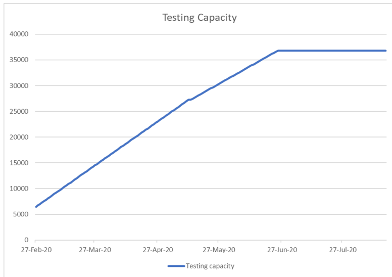
Figure S1. Testing capacity. The line graph shows scaling up of testing capacity over time taken into account in the model.
