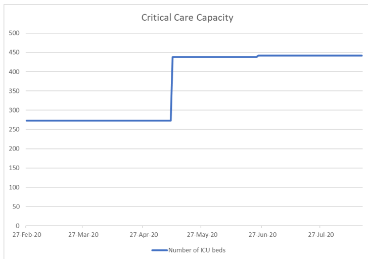
Figure S2. Critical care capacity. The graph shows change in critical care capacity over time taken into account in the model.
