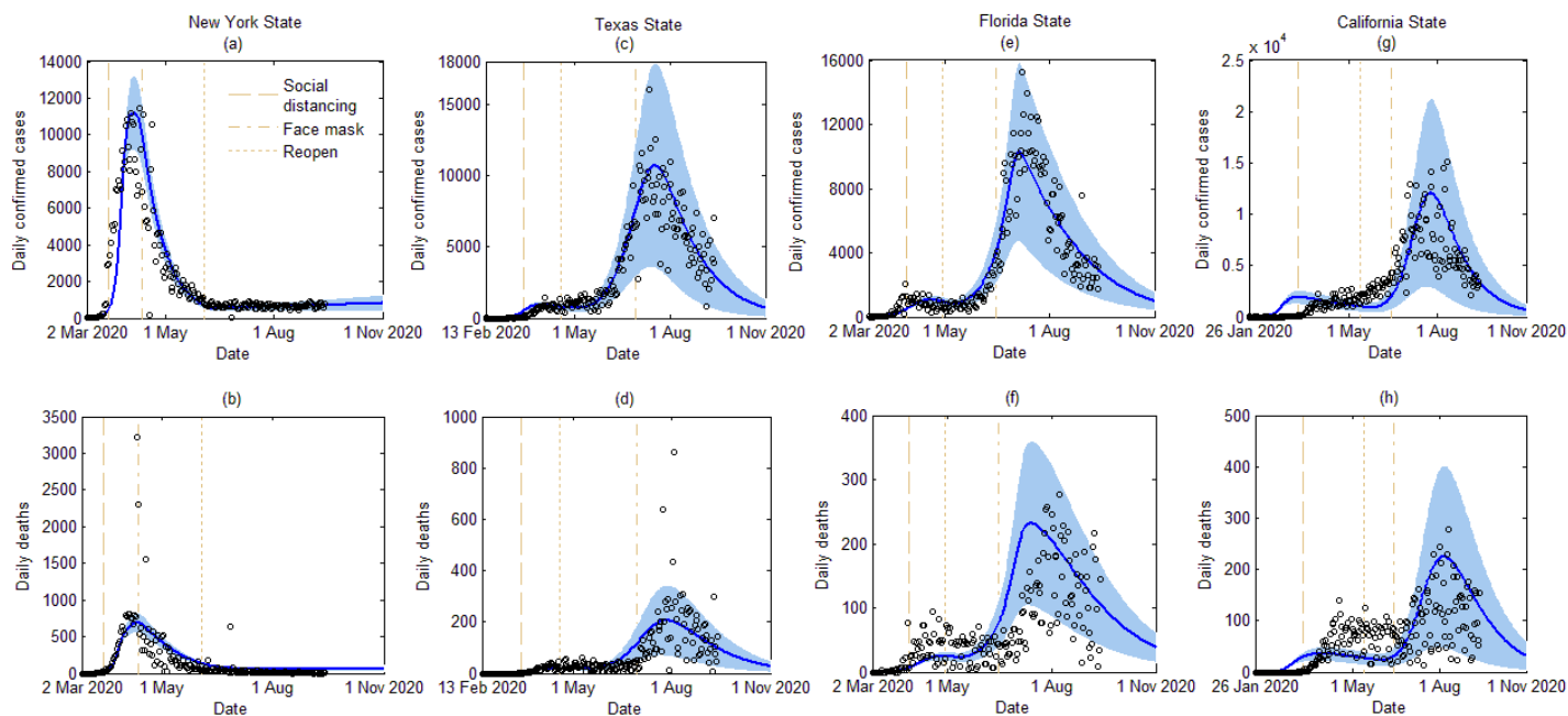
Figure 2. Model calibration and data fitting based on reported confirmed COVID-19 cases and deaths in four states, i.e., New York (a-b), Texas (c-d), Florida (e-f), and California (g-h). The blue areas denote 95% confidence intervals. Dashed lines, dash-dot lines, and dotted lines denote the social distancing order (public person-to-person contact rates decreased), face mask order, and reopening (public person-to-person contact rates recovered to no more than 100% of the pre-pandemic level) policies that were implemented in each state, respectively.
