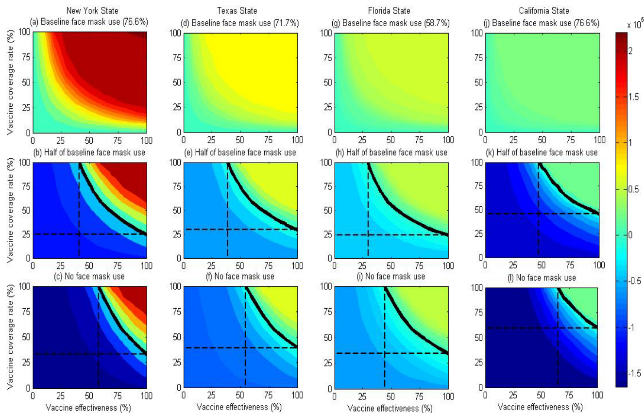
Figure 4. Contour plots of averted deaths as a function of vaccine effectiveness and vaccine coverage rate in four states when relaxing social distancing to pre-pandemic level and maintaining face mask use to the baseline level (the first line), half of the baseline level (the second line), and no use (the third line), compared with no vaccine. The black solid isoclines indicate the threshold that the number of averted deaths is zero. The black dashed lines correspond to the minimal vaccine effectiveness and vaccine coverage rate when the number of averted deaths is zero.
