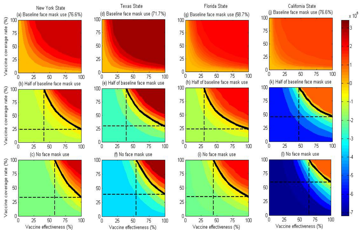
Figure 3. Contour plots of averted infections as a function of vaccine effectiveness and vaccine coverage rate in four states when social distancing is related to pre-pandemic level shortly after the commencement of vaccination. The first row is maintaining face mask use at baseline levels, the second row to reducing face masks use to half of the baseline level and the third row is no face mask use. The black solid isoclines indicate the threshold that the number of averted infections is zero. The black dashed lines correspond to the minimal vaccine effectiveness and vaccine coverage rate when the number of averted infections is zero.
