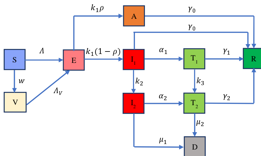
Figure 1. Flow chart of COVID-19 transmission model. The total population is divided into ten compartments (susceptible individuals (S), vaccinated individuals (V), latent infections (E), asymptomatic infections (A), undiagnosed infections with mild/moderate ( I_1 ) and severe/critical symptoms ( I_2 ), diagnosed infections with mild/moderate ( T_1 ) and severe/critical symptoms ( T_2 ), and recovered (R) and deceased (D) cases). The force of infection for susceptible and vaccinated individuals are denoted as \Lambda and \Lambda_V , which involves two transmission patterns: public settings (e.g., public transportation, supermarkets, offices, etc.) and households. The model includes three control measures: handwashing, social distancing and face mask use. More details on \Lambda and \Lambda_V are provided in the Appendix . The average incubation period is 1/k_1 , and the probability that an individual is asymptomatic is \rho . Infectious individuals with mild/moderate and severe/critical symptoms are diagnosed and treated at the rates \alpha_1 and \alpha_2 , respectively. We assume these diagnosed individuals are isolated strictly and could not further infect others. Undiagnosed and diagnosed mild/moderate cases progress to the severe/critical stage at the rates k_2 and k_3 , respectively. Asymptomatic infections and undiagnosed mild/moderate cases are assumed to recover naturally at the rate \gamma_0 . Diagnosed mild/moderate and severe/critical cases will recover at the rates \gamma_1 and \gamma_2 , respectively. Undiagnosed and diagnosed severe/critical cases will die due to the disease at the rates \mu_1 and \mu_2 , respectively. The vaccination rate is denoted as w .
