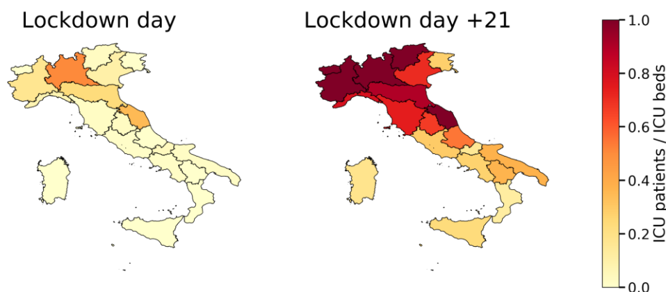
Figure 5. Spatial distribution of COVID-19 ICU patients in Italy. The maps represent the ICUs saturation (number of ICU patients divided by number of ICU beds) at the regional level on March 9 th (left panel), when the lockdown was imposed, and twenty-one days later, on March 30 th (right panel). Here we use the regional number of ICU beds reported before the onset of the epidemic. The number of ICU beds was increased throughout the epidemic.
