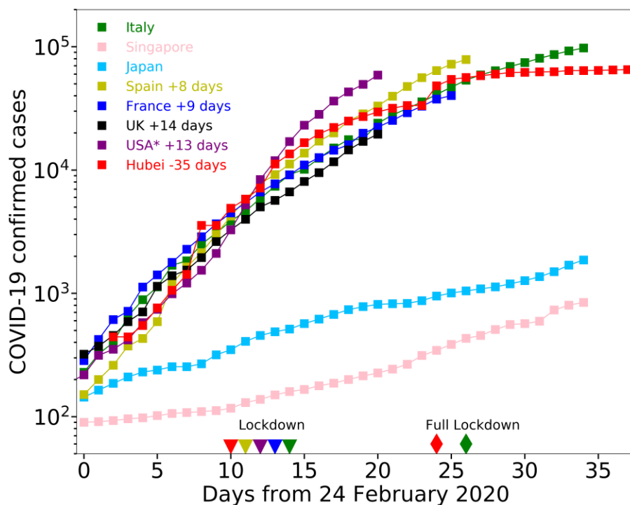
Figure 1. Number of confirmed COVID-19 cases for different countries. Trajectories are shifted temporally to superpose one on another, so that day zero represents the onset of COVID-19 outbreak for all countries. Japan and Singapore were able to contain the outbreak at the very early stage. The Chinese region of Hubei was able to contain diffusion at a later stage, by imposing first a milder lockdown of the population on January 30 th 2020 (red triangle), and then a full lockdown of the population on February 13 th 2020 (red diamond), closing all non-essential companies and manufacturing plants. Italy, Spain, France, UK, and the American States of California and New York (referred as US*) display exponential growth of confirmed cases. Italy, Spain, France and US* imposed the lockdown at similar (relative) times, indicated by the green, gold, blue and purple triangles, respectively. The four countries have comparable population sizes to Hubei region (58.5M people), with the minimum in Spain (46.7M people)
