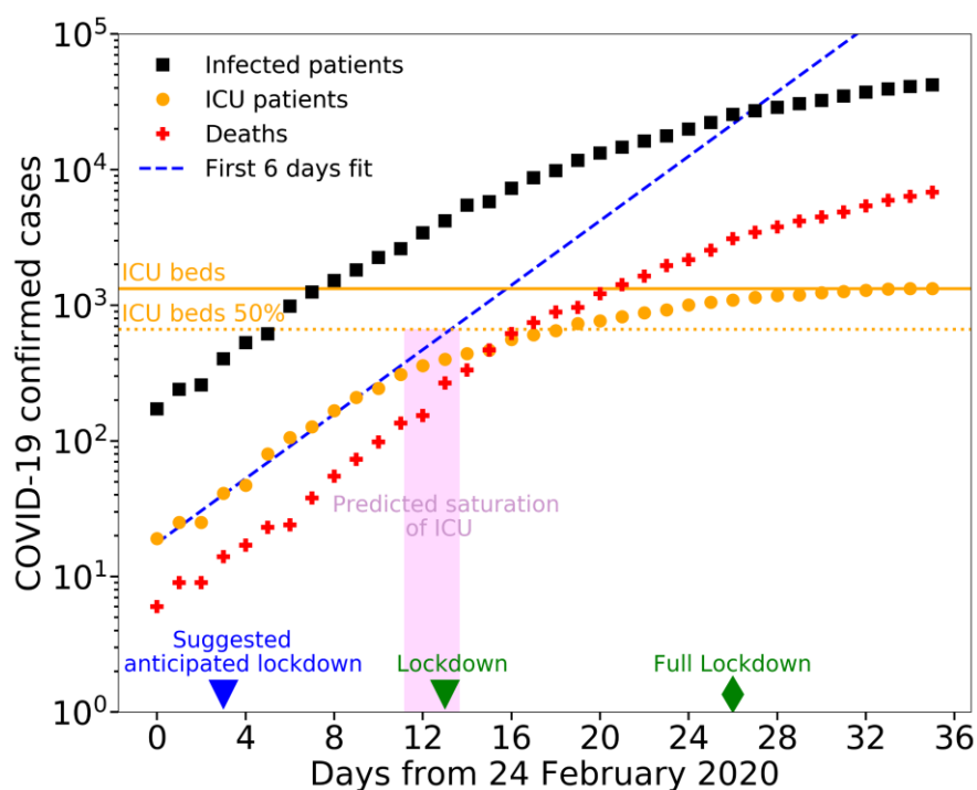
Figure 4. The date of ICUs saturation can be predicted early on. The number of deaths (red crosses) grows exponentially in time in Lombardy region, Italy. The number of ICU patients (orange circles) flattens in time: this indicates the saturation of the ICU beds in the region. The dotted blue line is the linear regression of the first six orange data points. The day of the saturation can be predicted by linear regression, fitting the logarithm of the number of ICU patients at early stages of the epidemic: the timeline highlighted in magenta shows the predicted temporal range for the saturation of 50% of the ICU beds; the beginning and the end of the magenta range are obtained by fitting the first four (blue triangle) and nine orange data points respectively. To avoid ICUs saturation, an earlier lockdown (indicated by the blue triangle) would have been necessary. The green triangle and green diamond represent the lockdown day (March 8 th 2020) and full lockdown day (March 21 st 2020). The orange solid line and dotted line represent 100% and 50% of the actual total number of ICU beds in Lombardy.
